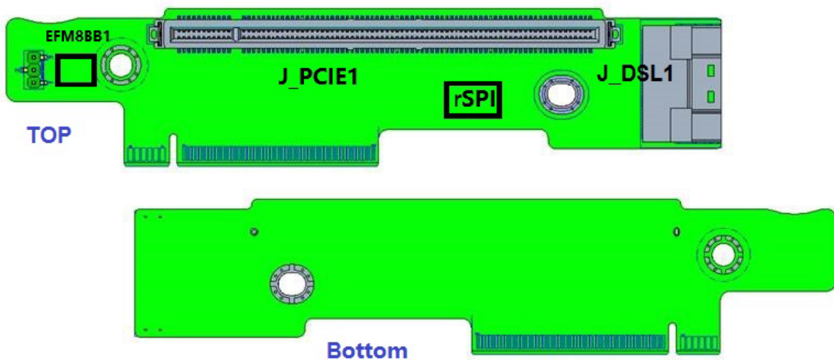
Figure 6. Riser 1B dimension
