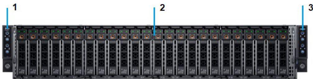
Figure 1. Front view of the C6400 Chassis
