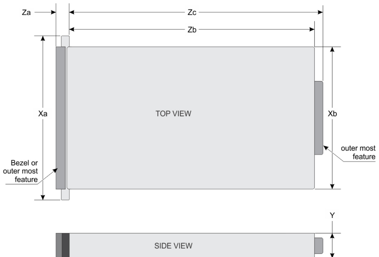
Figure 19. C6400 Chassis dimensions
