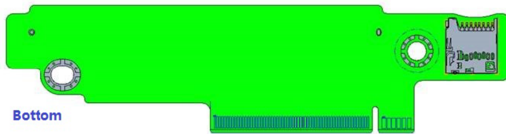
Figure 5. Riser 1A dimension
