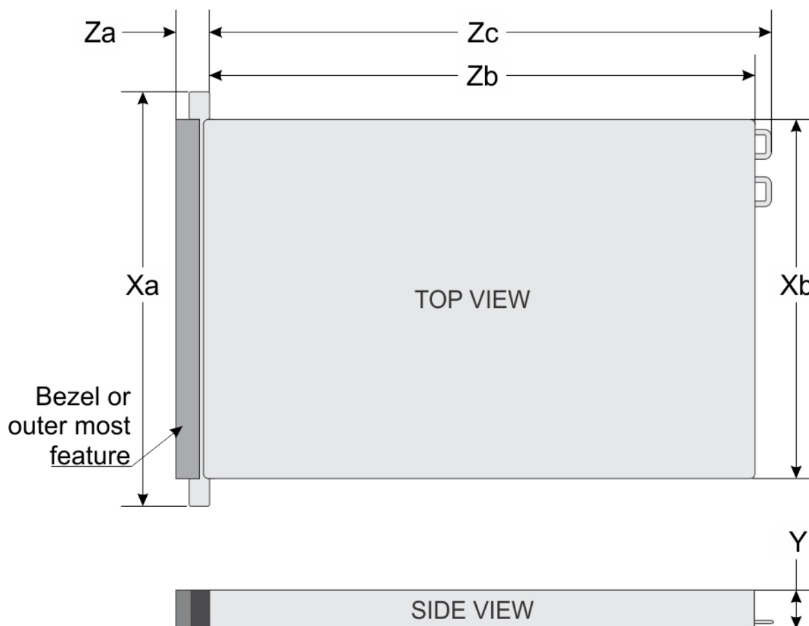
Figure 1. PowerEdge R250 Chassis dimensions
