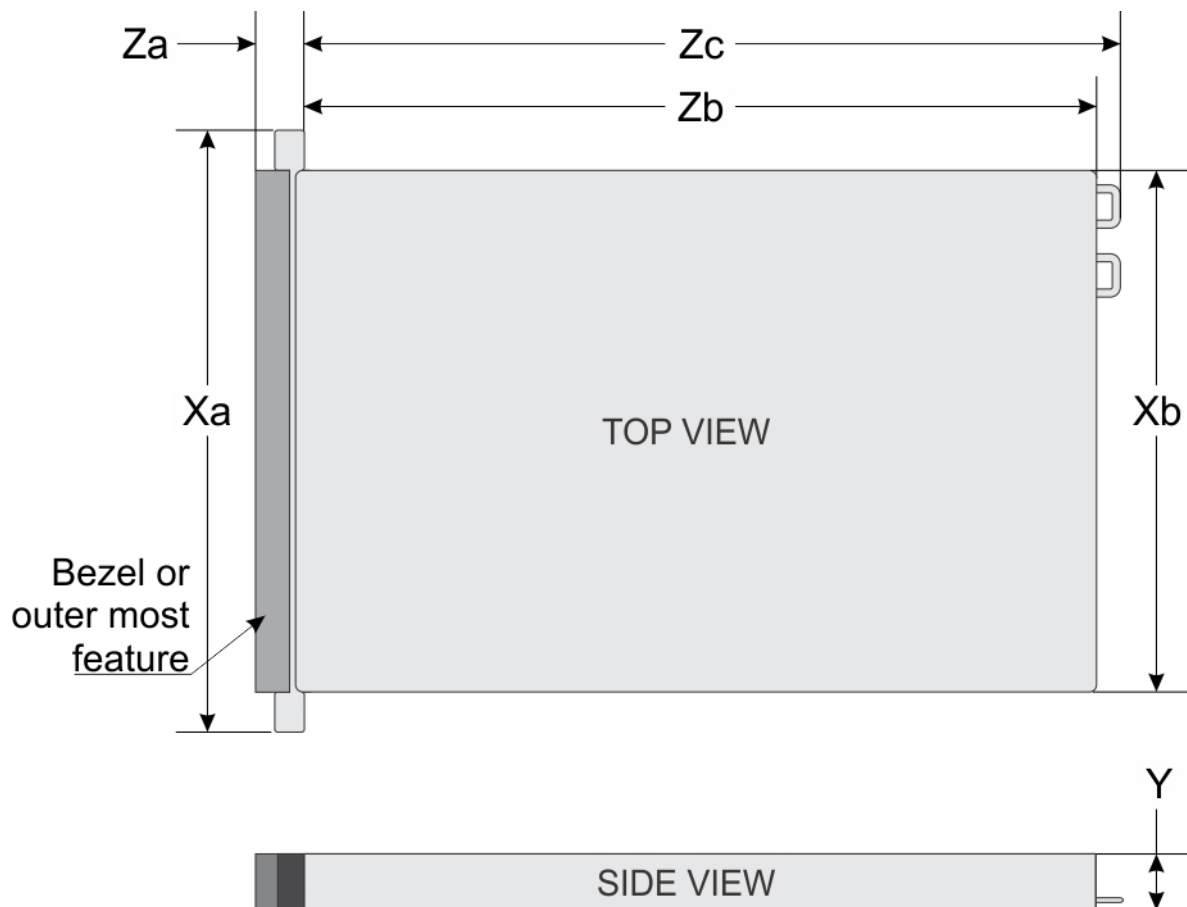
Figure 1. Chassis dimensions
