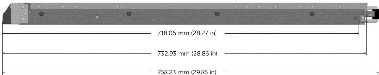
Figure 24. Chassis depth without bezel for 8-drive chassis option
