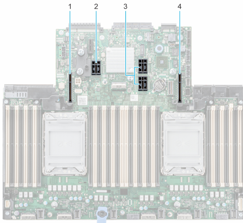
Figure 119. Expansion card slot connectors
