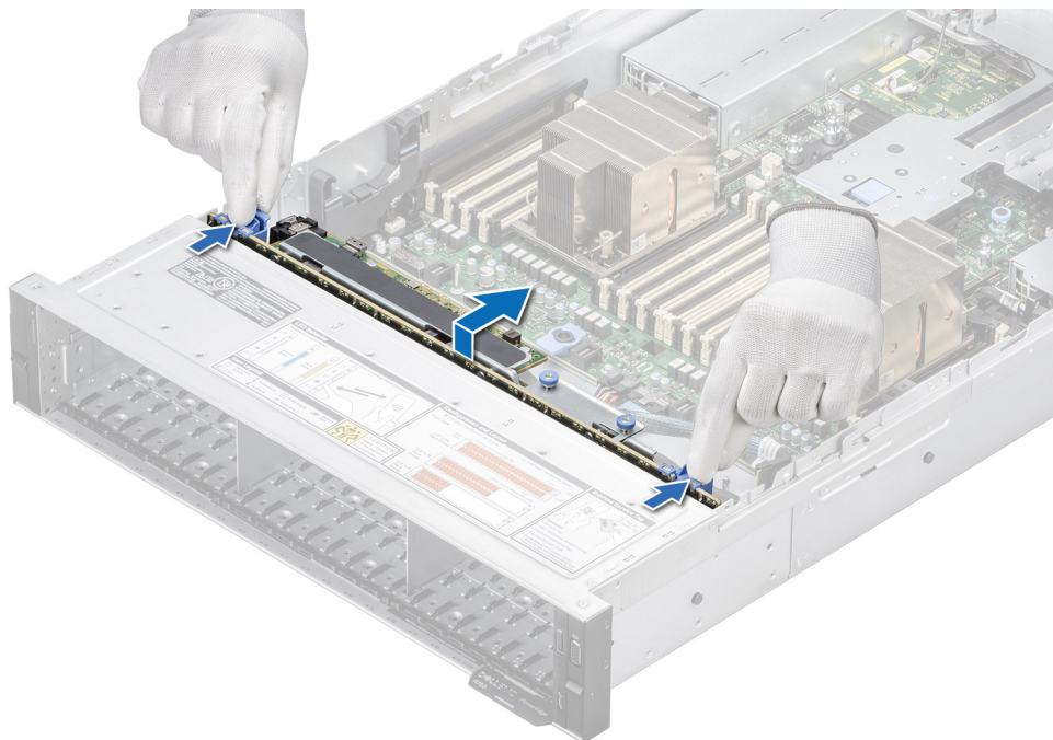
Figure 66. Removing the drive backplane
