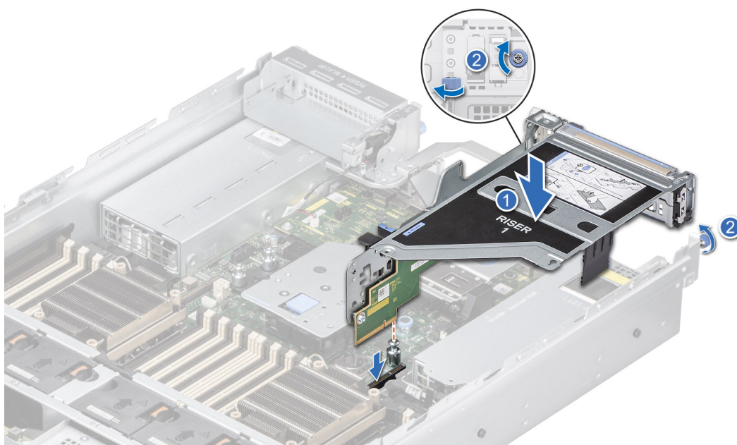
Figure 146. Installing the expansion card riser (Riser 1)
