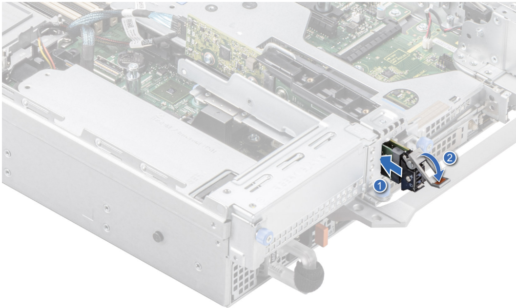
Figure 197. Installing the BOSS S2 card carrier
