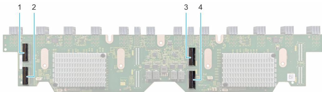
Figure 65. 24 x 2.5-inch NVMe switched board
