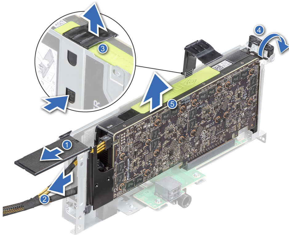
Figure 163. Removing GPU from Riser 4
