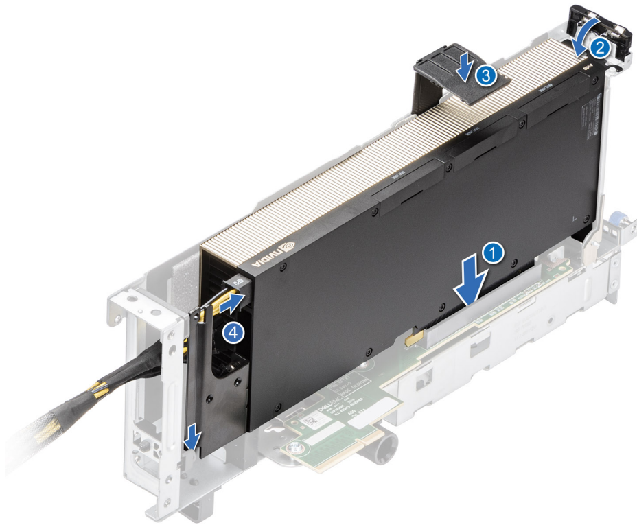
Figure 166. Installing GPU on Riser 1
