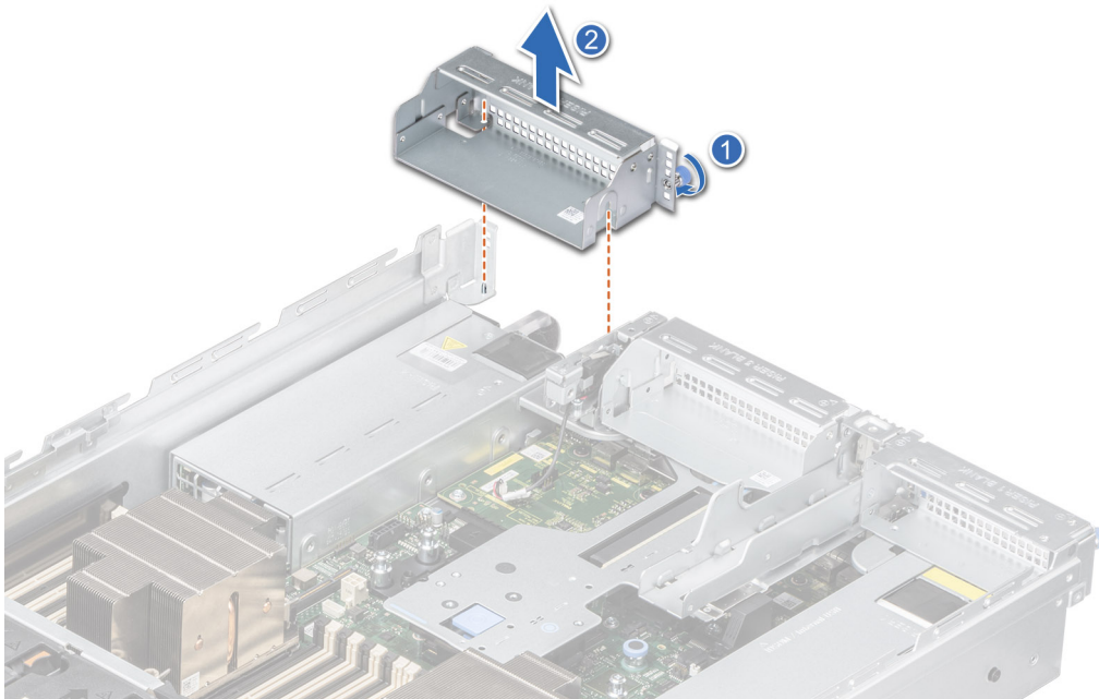
Figure 159. Removing the Riser 4 blank
