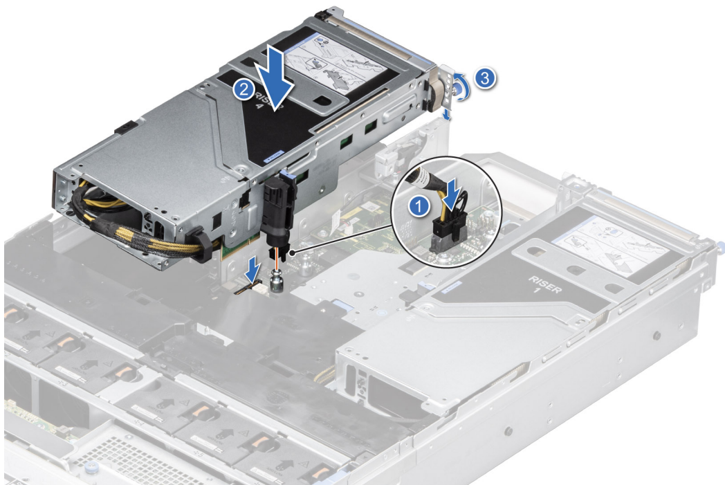
Figure 161. Installing the expansion card riser (Riser 4)
