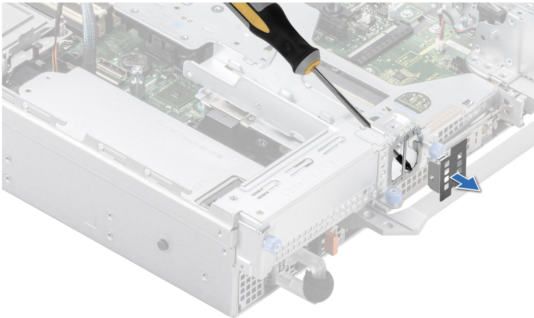
Figure 230. Removing the BOSS S2 module blank
