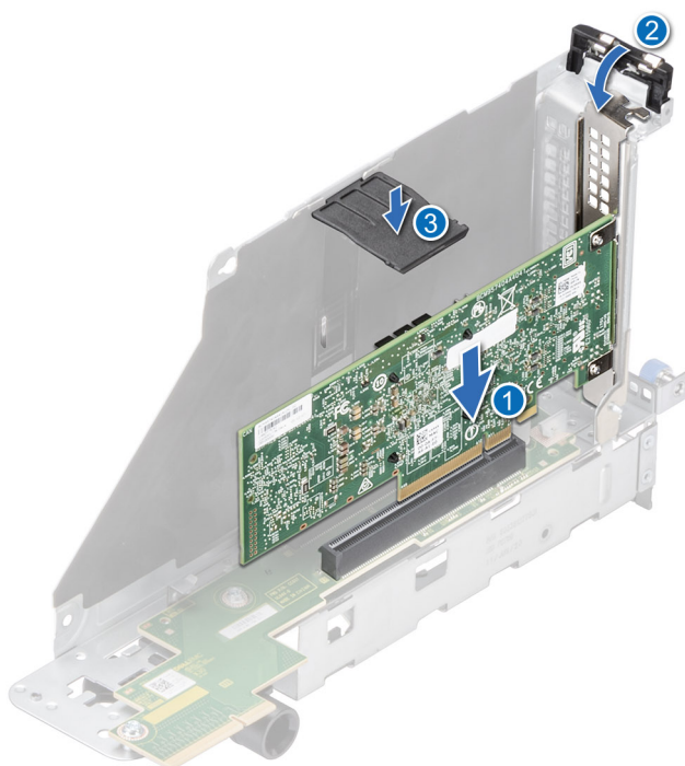
Figure 152. Installing an expansion card into the expansion card riser
