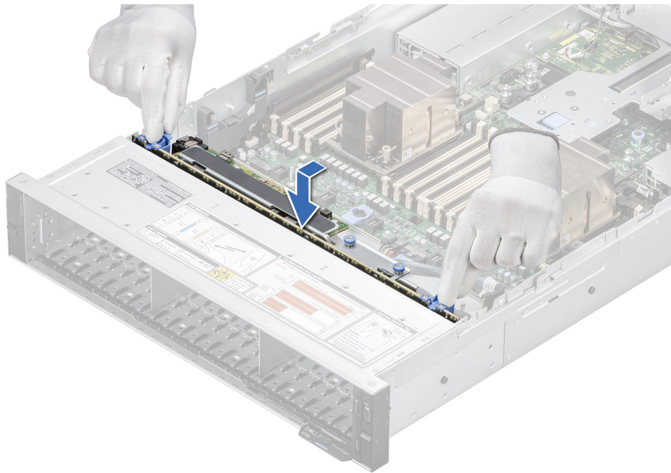
Figure 67. Installing the drive backplane
