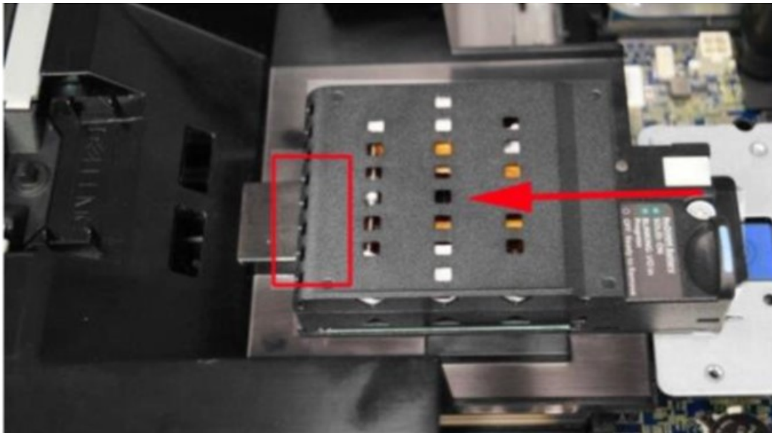
Figure 239. Installing the battery on the air shroud
