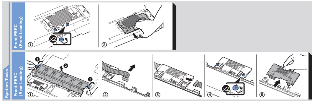
Figure 21. System tasks
