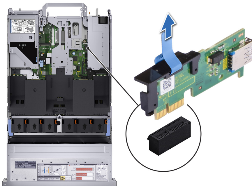
Figure 200. Removing the internal USB card
