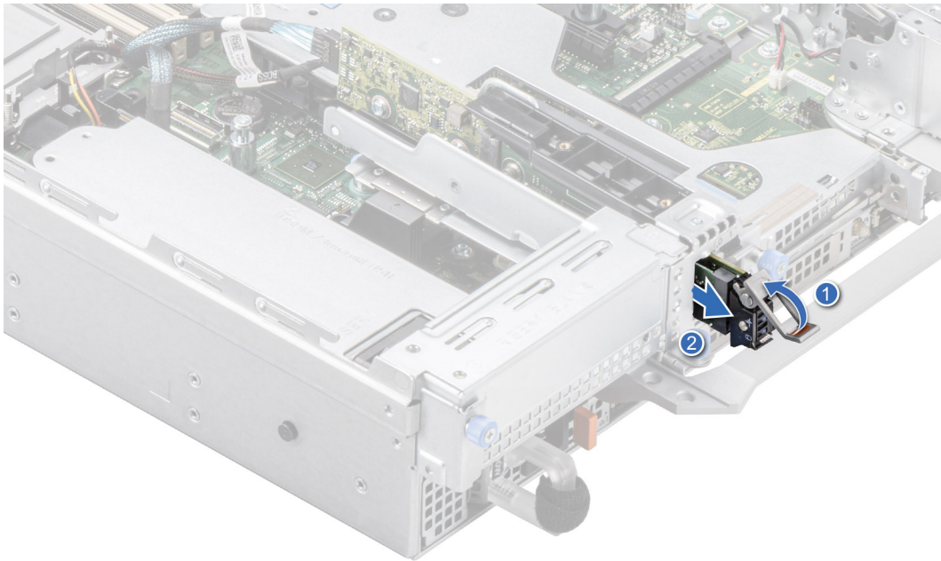
Figure 190. Removing the BOSS S2 card carrier
