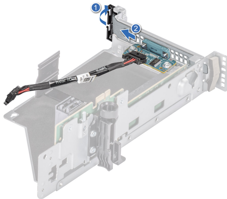
Figure 175. Removing the Serial COM port
