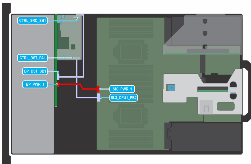
Figure 79. 16 x 2.5-inch SAS/SATA with fPERC
