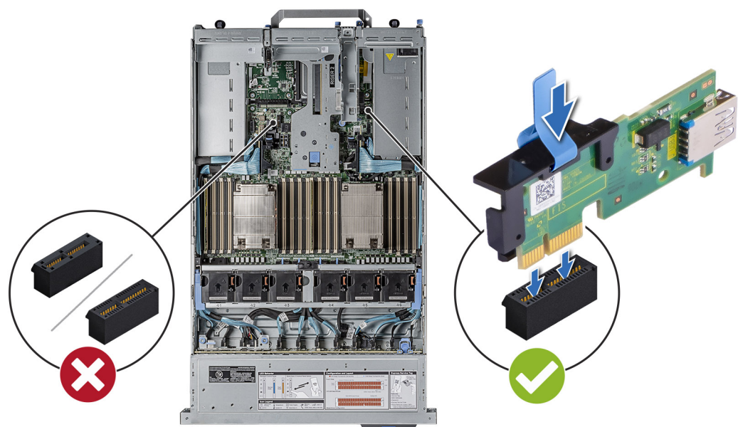
Figure 234. Internal USB card port information
