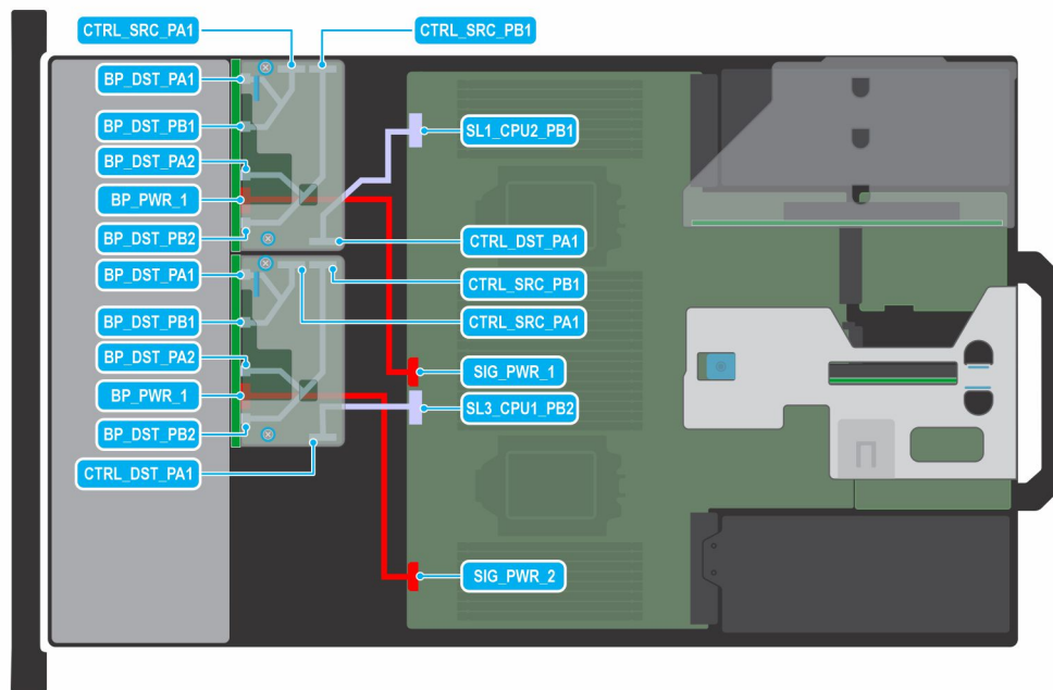
Figure 78. 16 x 2.5-inch NVMe with fPERC
