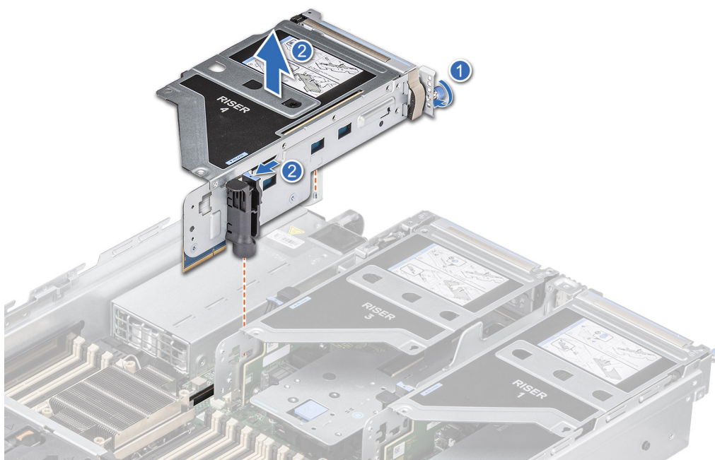
Figure 136. Removing the expansion card riser (Riser 4)
