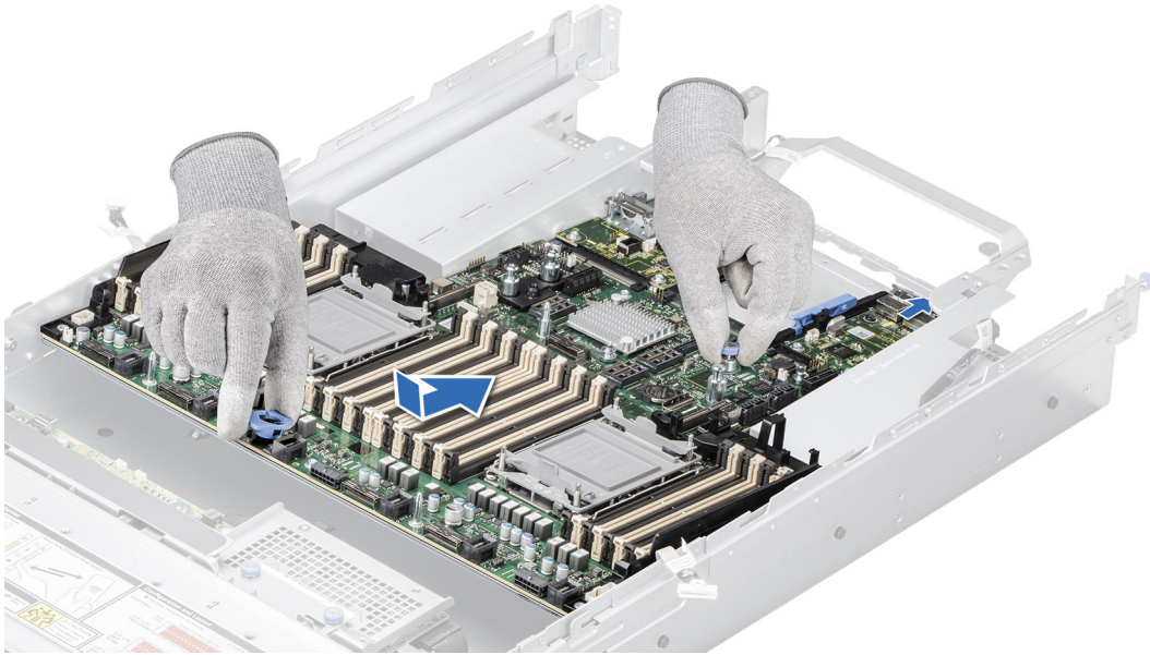
Figure 220. Installing the system board
