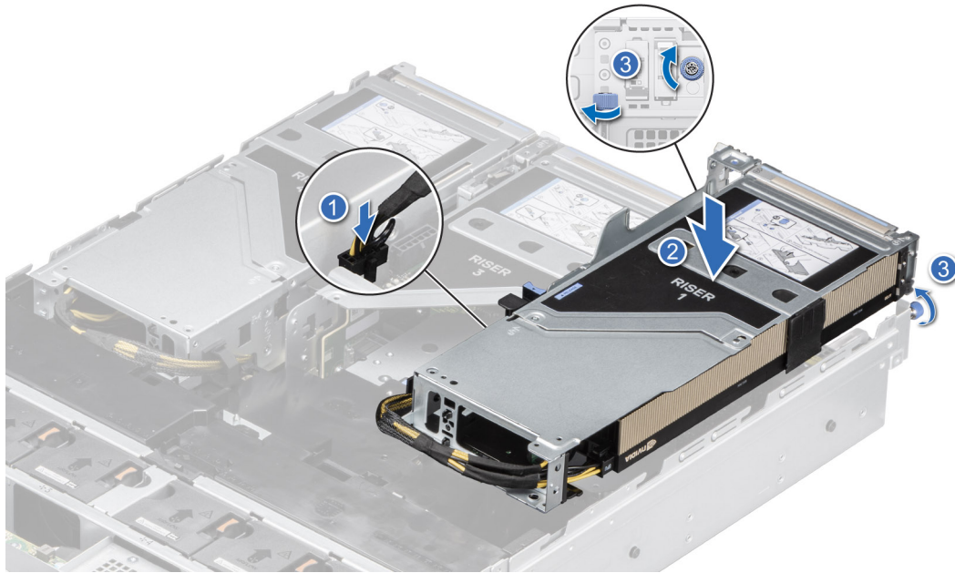
Figure 160. Installing the expansion card riser (Riser 1)
