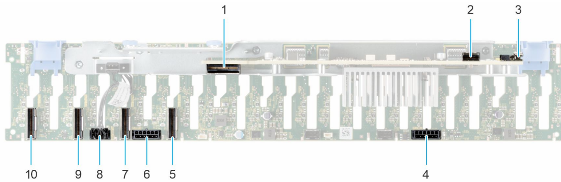
Figure 63. 24 x 2.5-inch drive backplane
