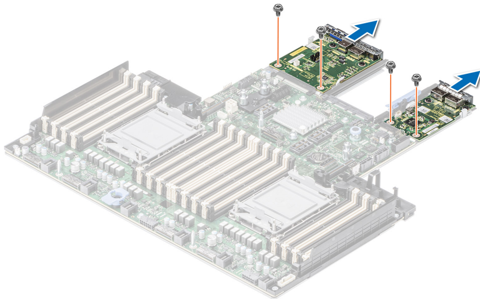
Figure 221. Removing the LOM card and rear I/O board
