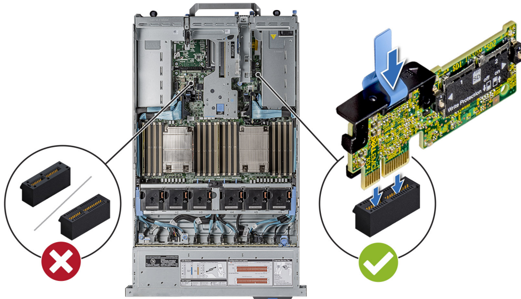
Figure 233. IDSDM port information
