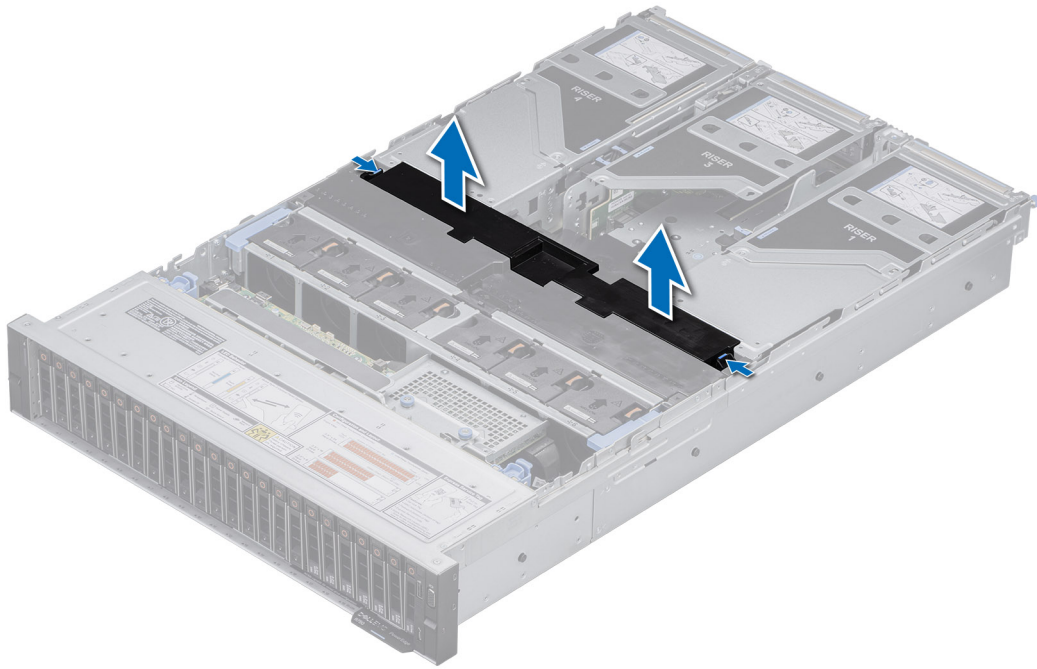
Figure 35. Removing the GPU air shroud top cover
