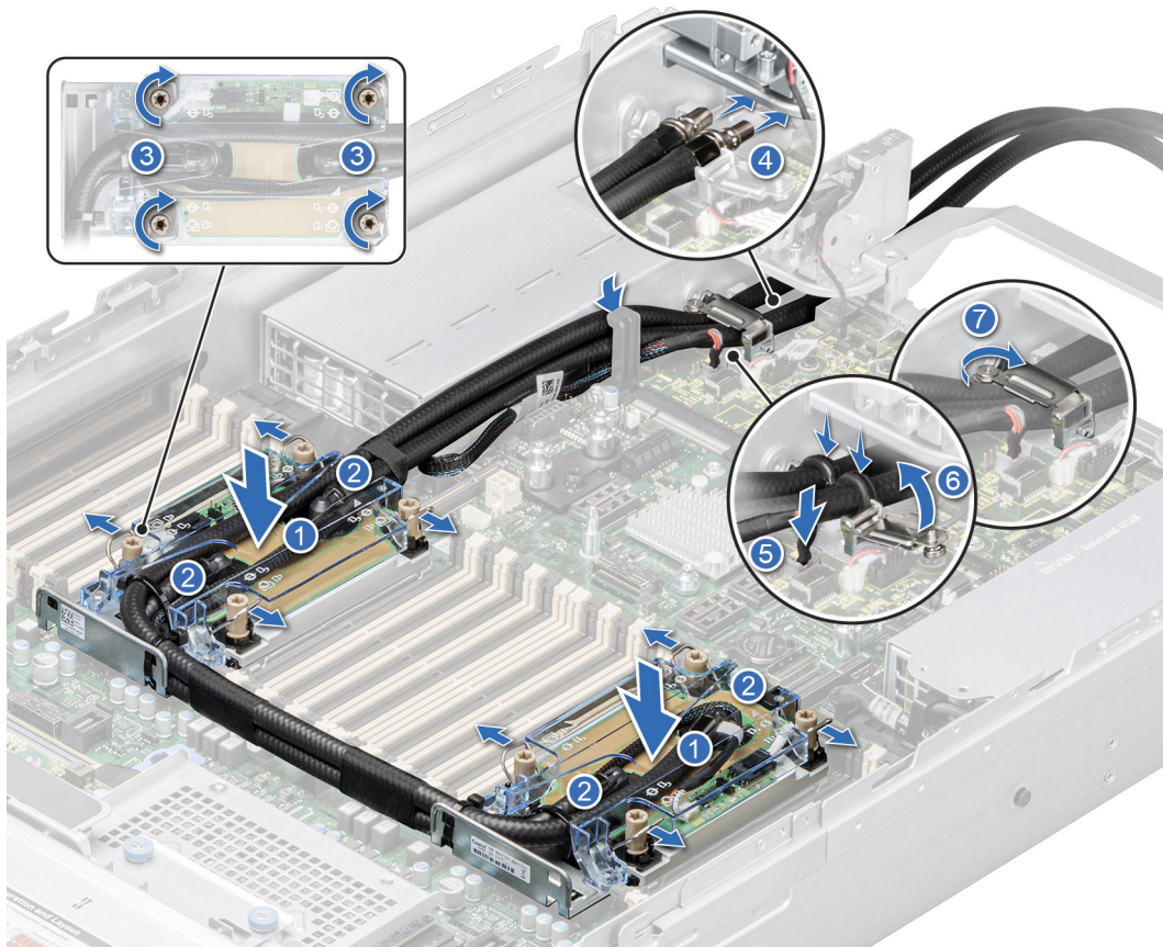
Figure 118. Installing the liquid cooling module
