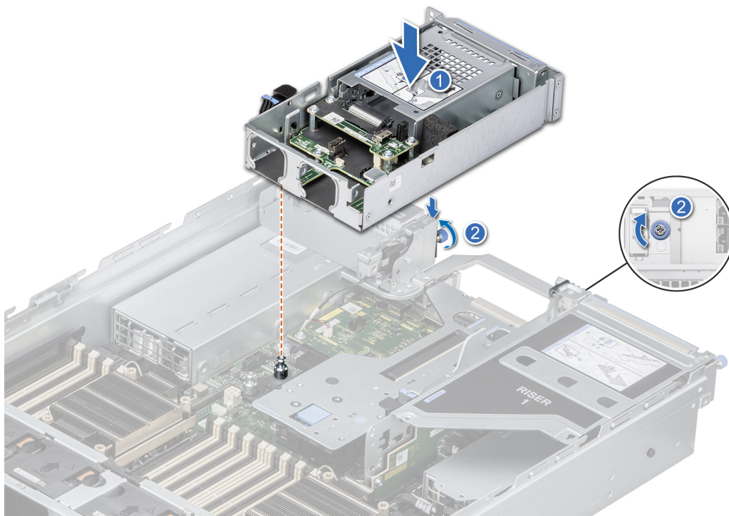
Figure 59. Installing the 2 x 2.5-inch rear drive module
