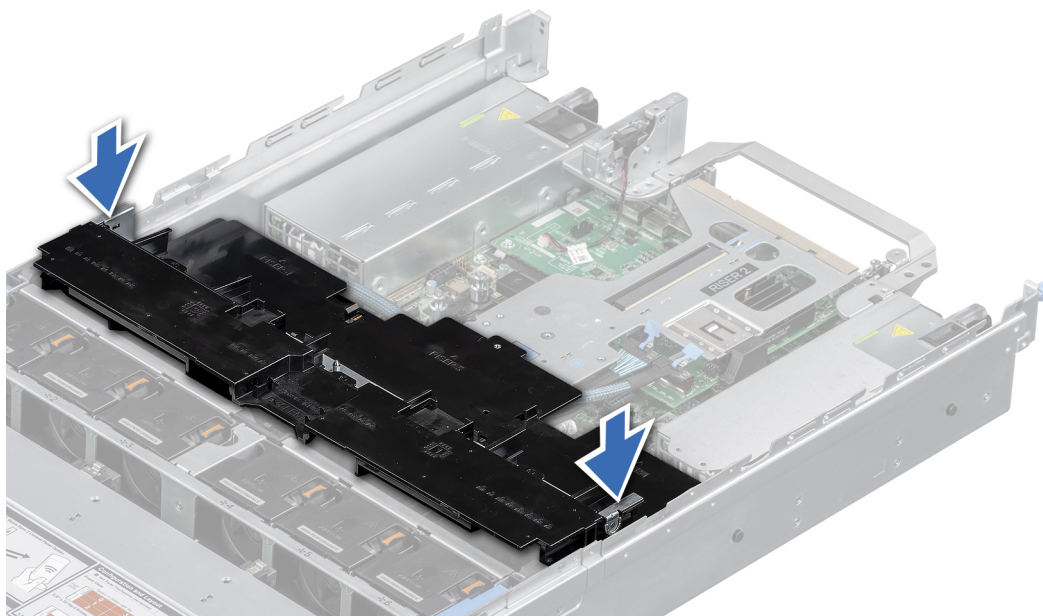
Figure 34. Installing the GPU air shroud
