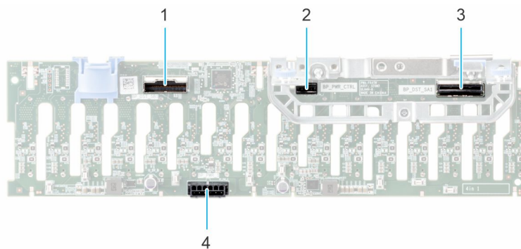
Figure 62. 16 x 2.5-inch drive backplane
