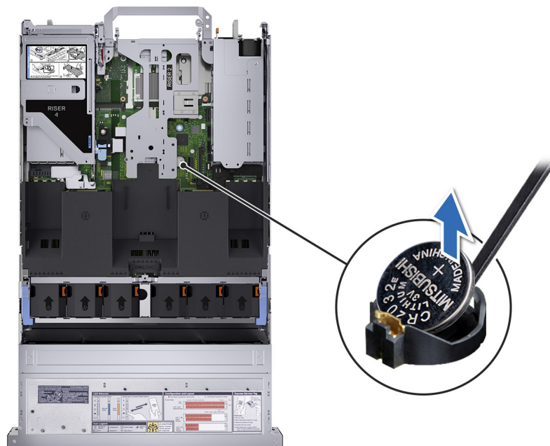
Figure 198. Removing the system battery
