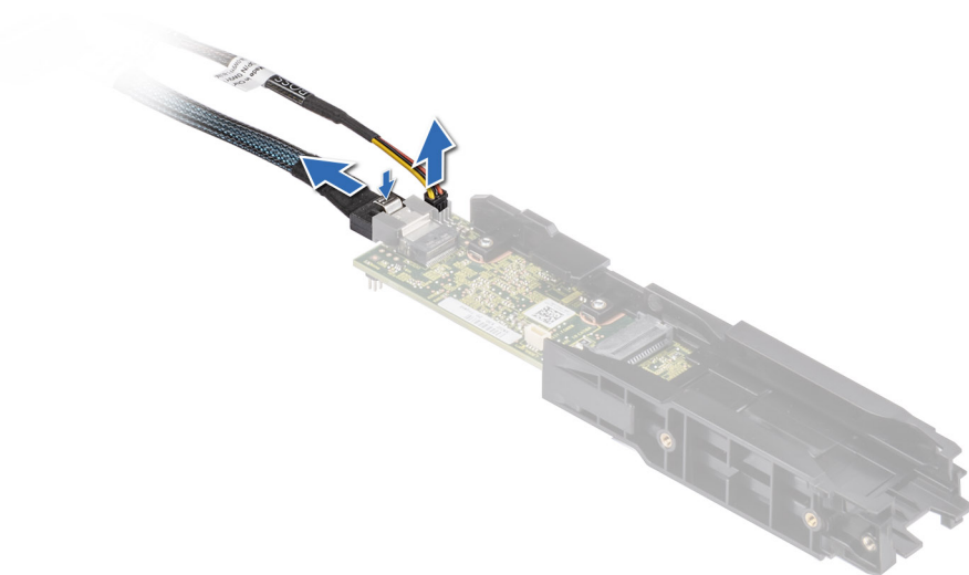
Figure 193. Removing the BOSS S2 power and signal cable from the BOSS S2 module
