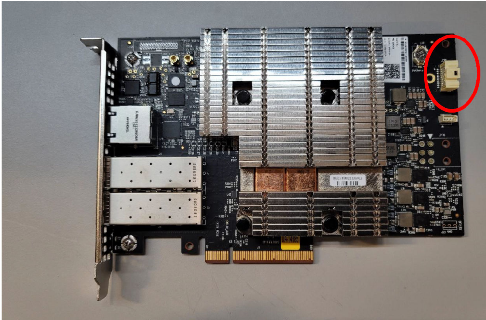
Figure 235. Front View of the DPU card
