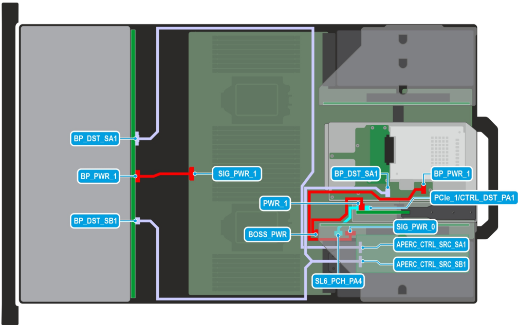
Figure 68. 12x 3.5-inch SAS/SATA + 2 x 2.5-inch SAS/SATA with APERC in Riser 1 and optional BOSS S2 module
