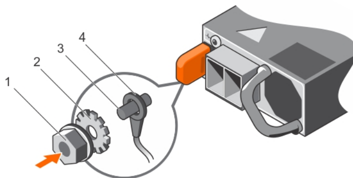
Figure 214. Assembling and connecting the safety ground wire
