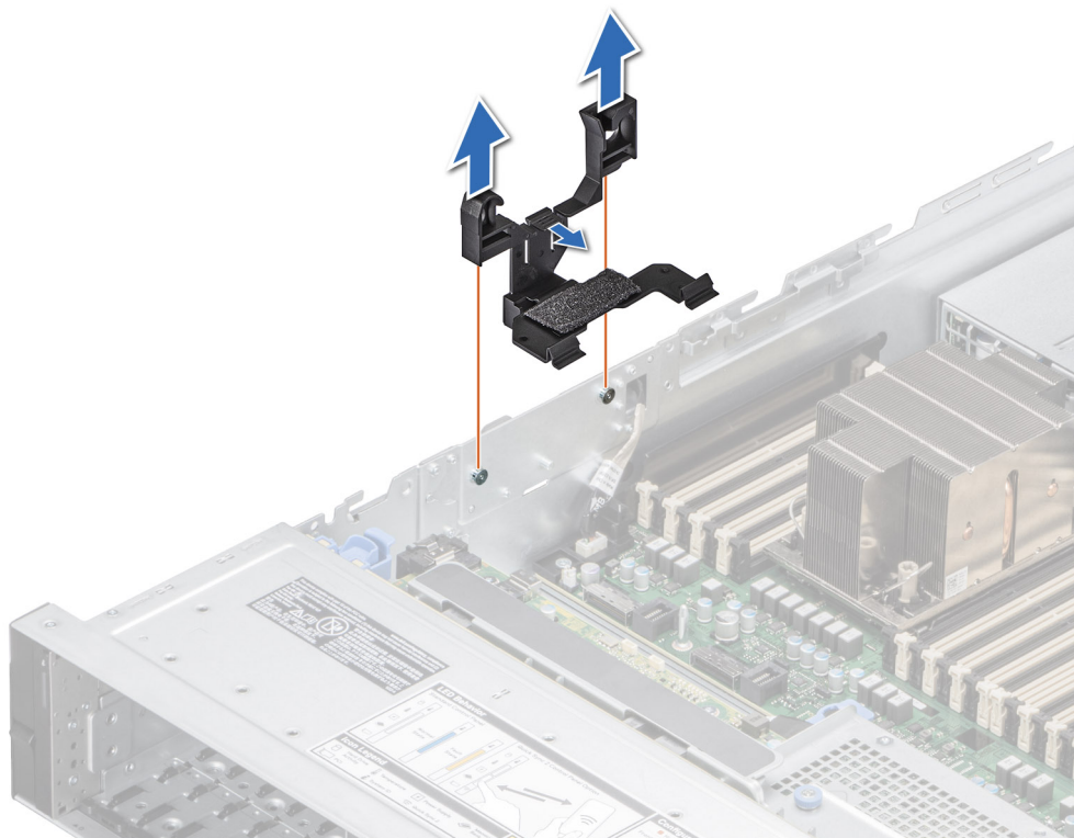
Figure 47. Removing the side wall bracket
