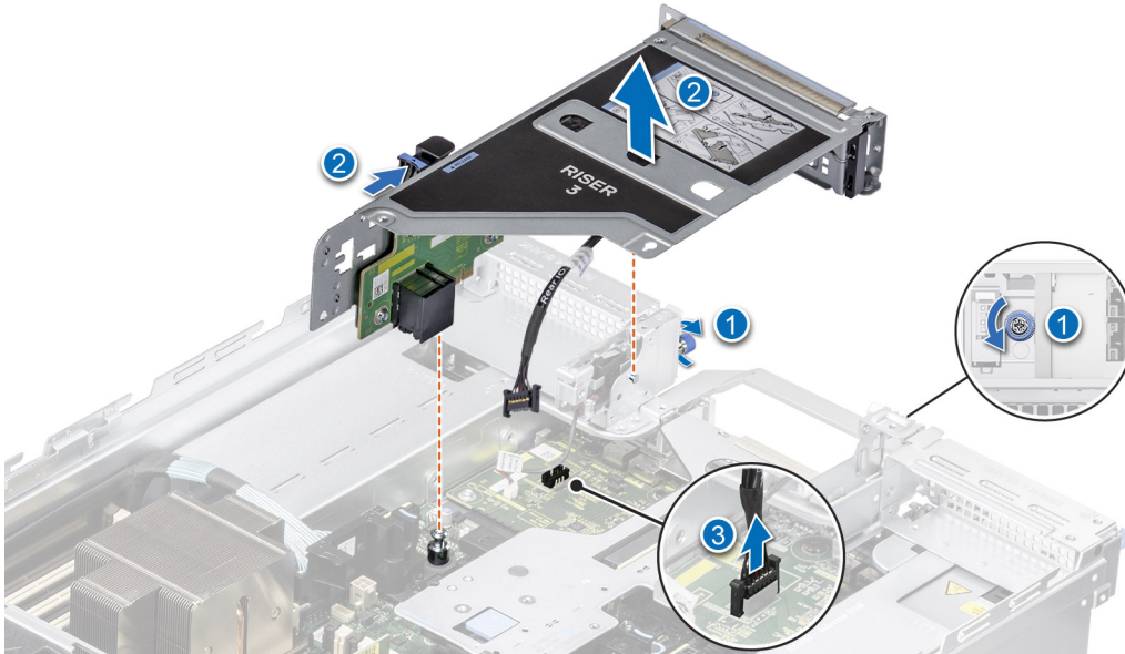
Figure 174. Disconnecting the serial COM port
