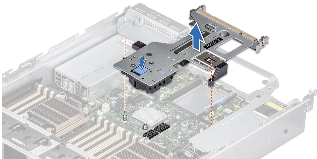
Figure 135. Removing the expansion card riser (Riser 2)
