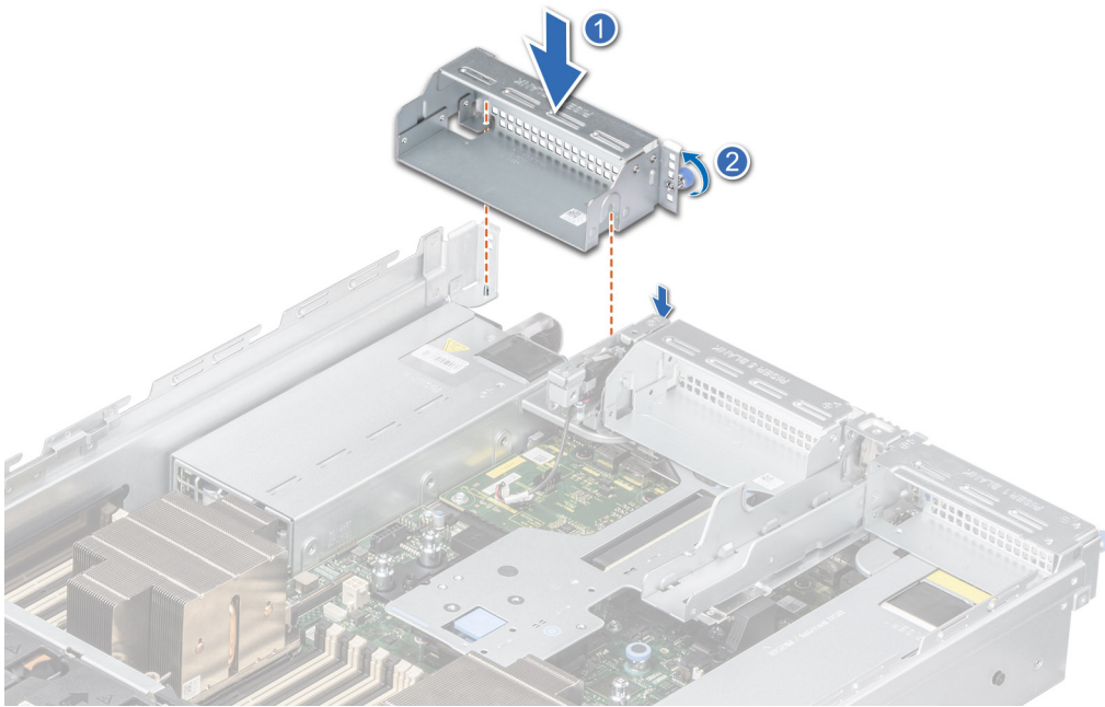
Figure 140. Installing the Riser 4 blank
