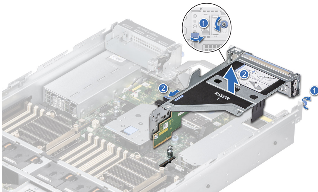
Figure 133. Removing the expansion card riser (Riser 1)
