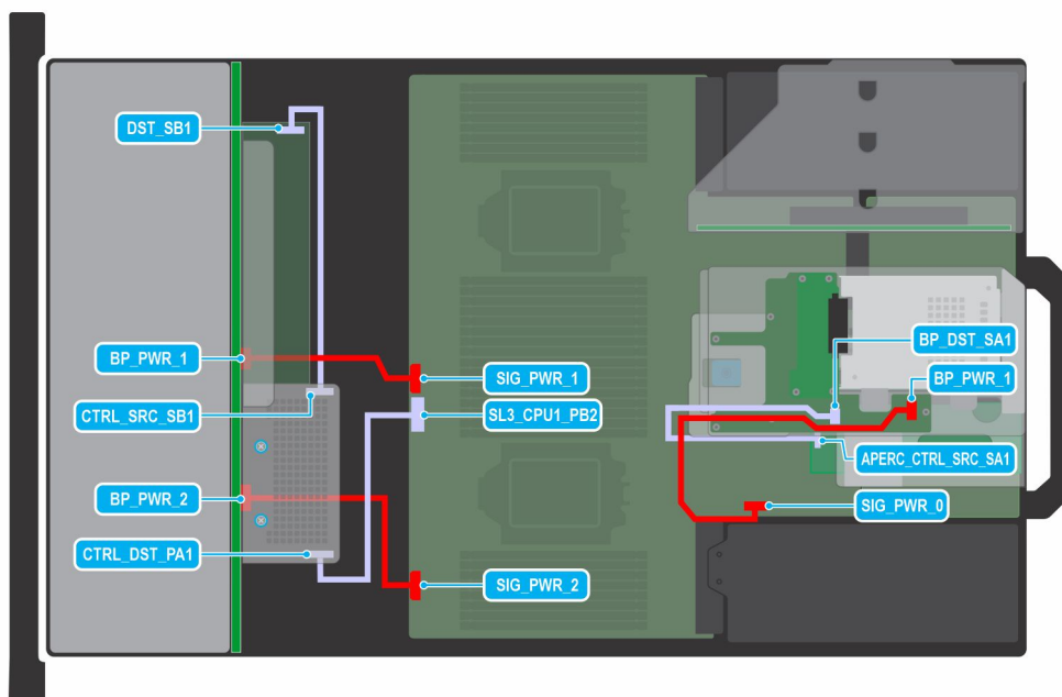
Figure 92. 24 x 2.5-inch SAS/SATA with separate controller, expander, APERC in R2, and fPERC
