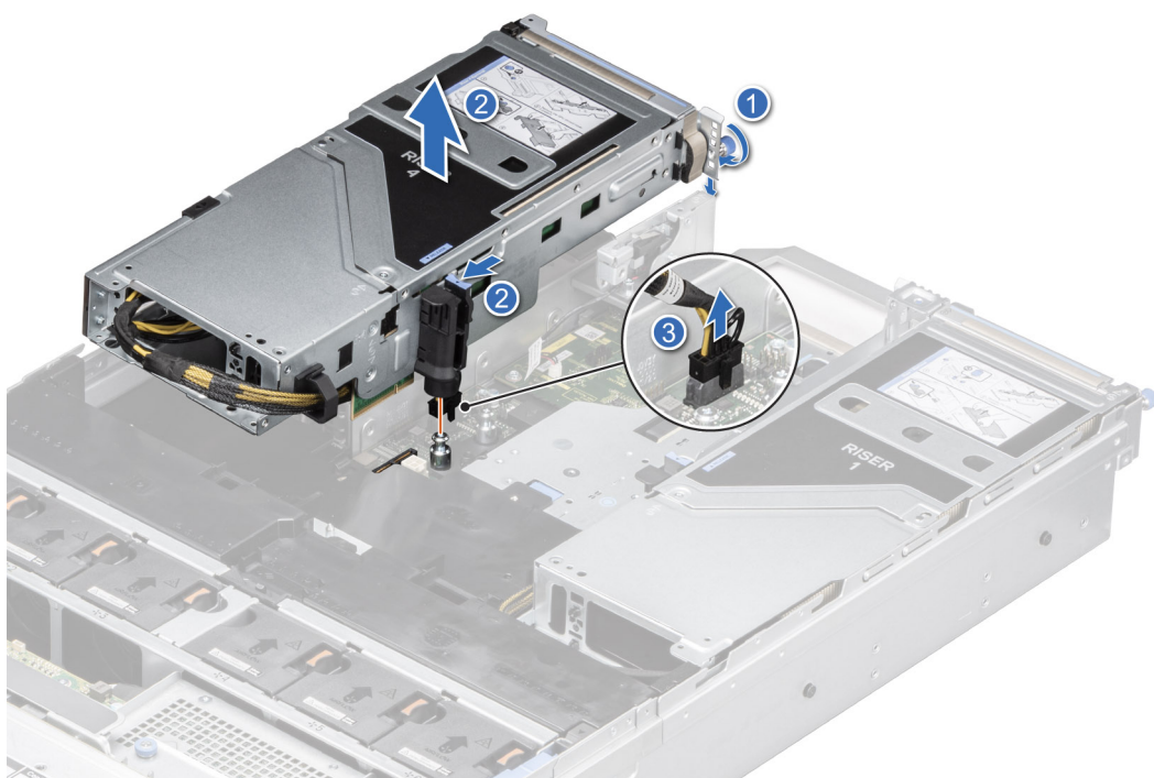
Figure 155. Removing the expansion card riser (Riser 4)
