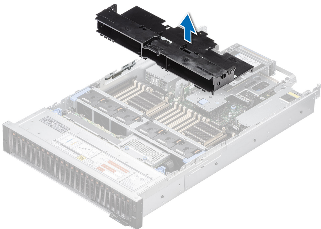
Figure 33. Removing the GPU air shroud
