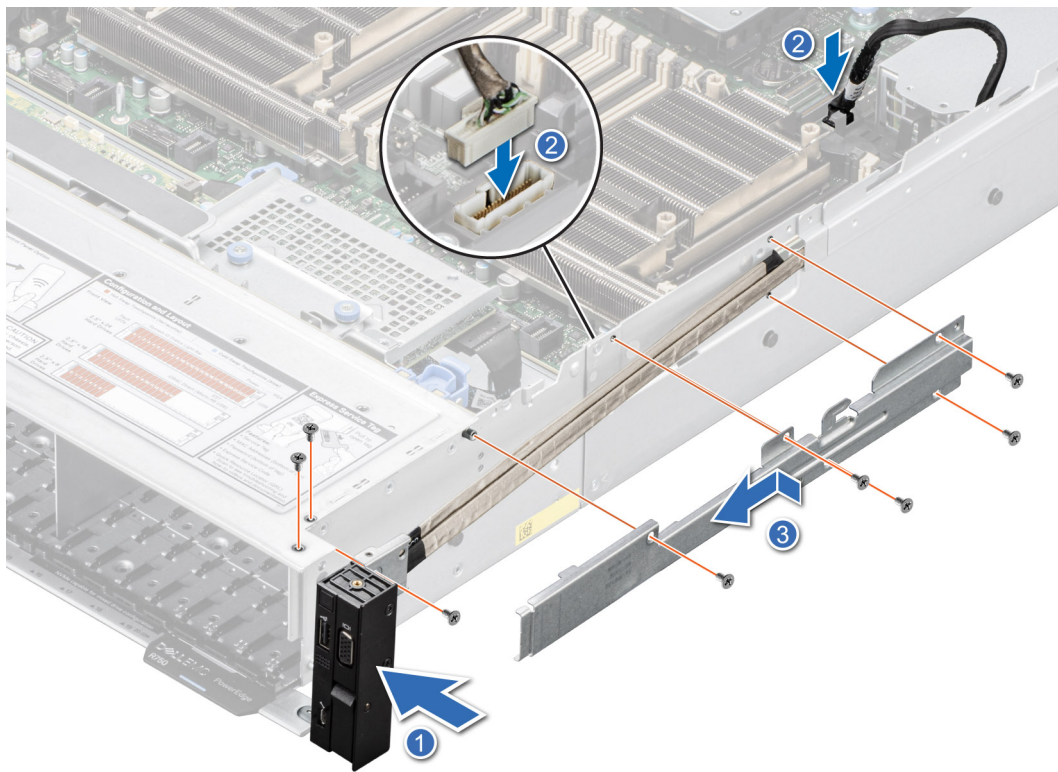
Figure 226. Installing the right control panel
