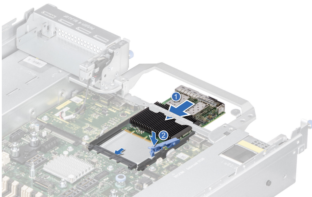
Figure 207. Installing the OCP card
