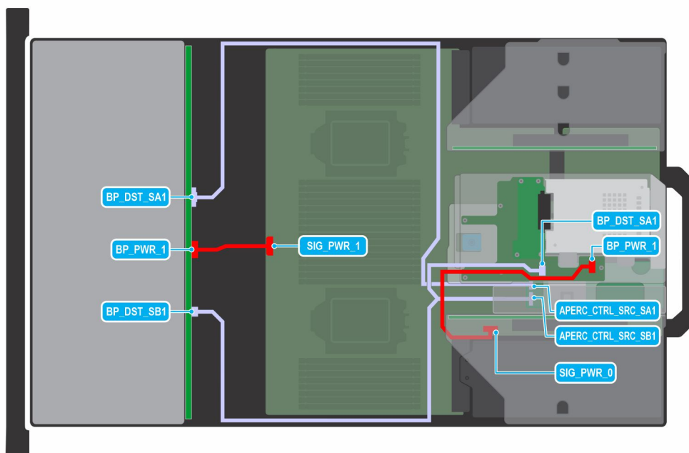
Figure 69. 12 x 3.5-inch SAS/SATA + 2 x 2.5-inch SAS/SATA with APERC in Riser 2
