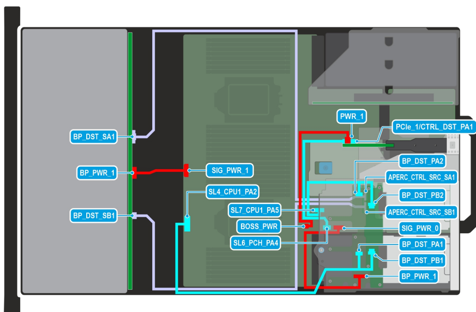
Figure 73. 12 x 3.5-inch SAS/SATA + 4 x 2.5-inch NVMe with APERC in Riser 2 and optional BOSS S2 module
