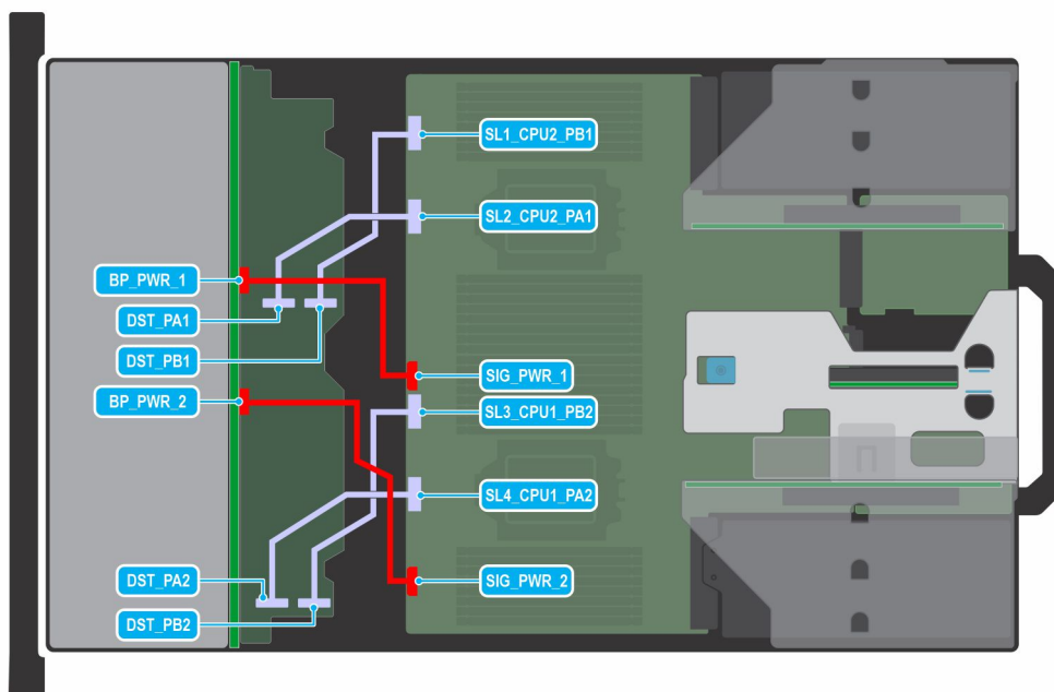
Figure 93. 24 x 2.5-inch NVMe switch
