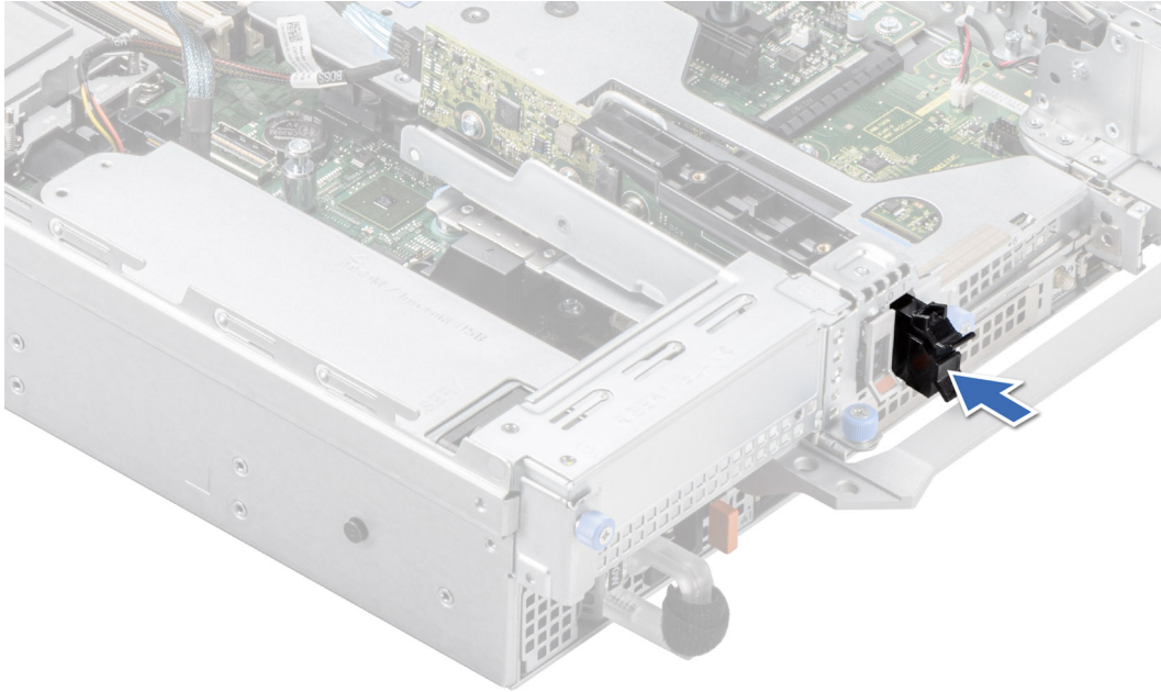
Figure 189. Installing the BOSS S2 card carrier blank
