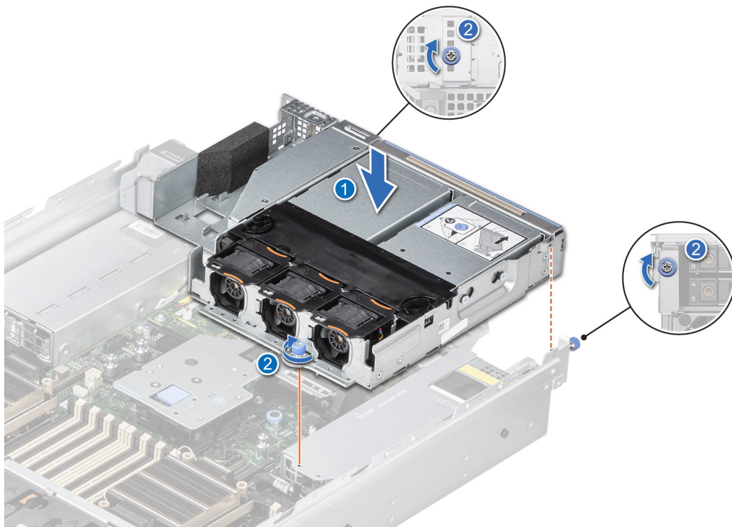
Figure 57. Installing the 4 x 2.5-inch rear drive module
