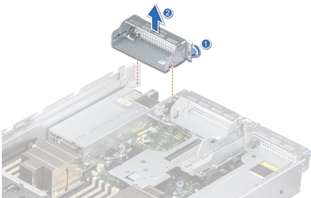
Figure 144. Removing the Riser 4 blank
