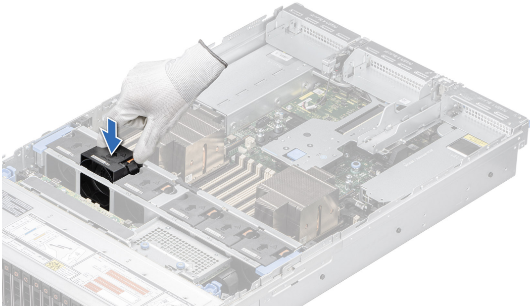
Figure 44. Installing a cooling fan
