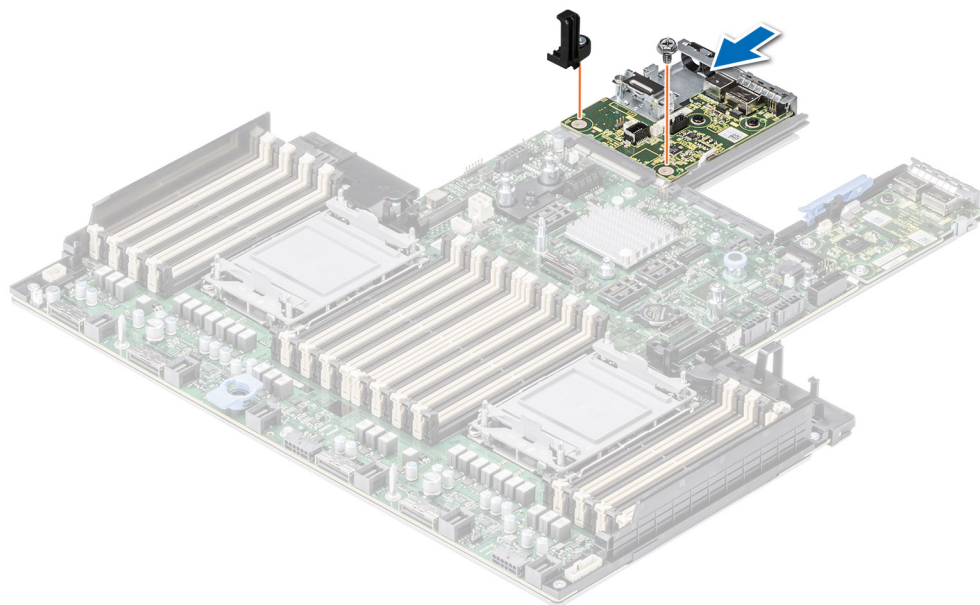
Figure 224. Installing the liquid cooling rear I/O board
