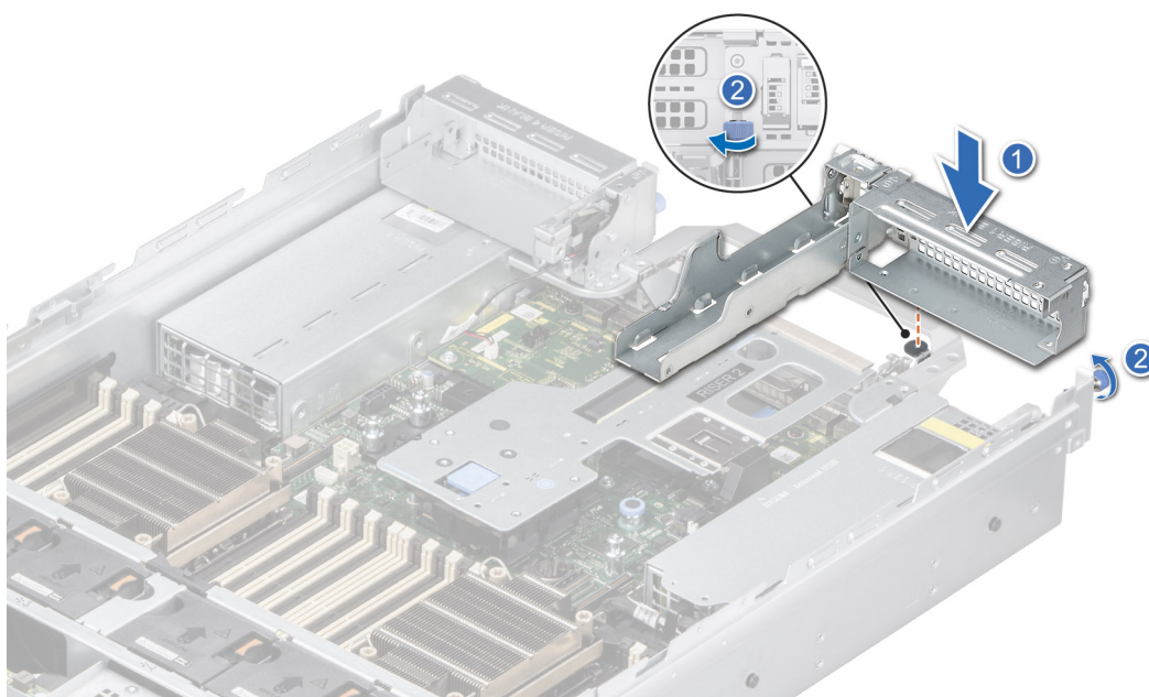
Figure 137. Installing the Riser 1 blank
