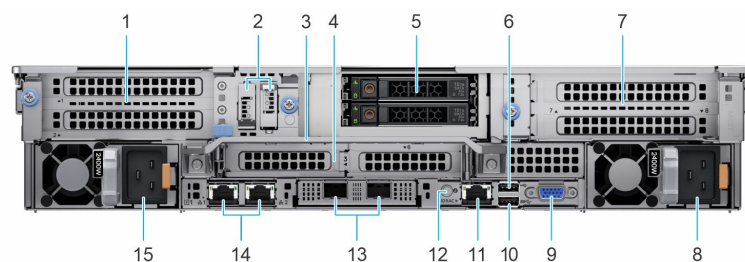
Figure 9. Rear view of the system with 2 x 2.5-inch rear drive module
