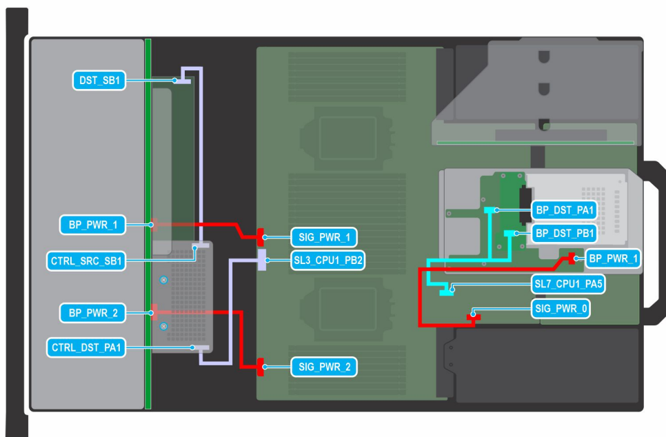
Figure 88. 24 x 2.5-inch SAS/SATA + 2 x 2.5-inch NVMe with expander and fPERC
