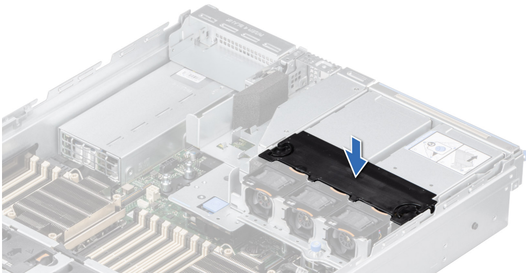
Figure 40. Installing the rear drive module air shroud
