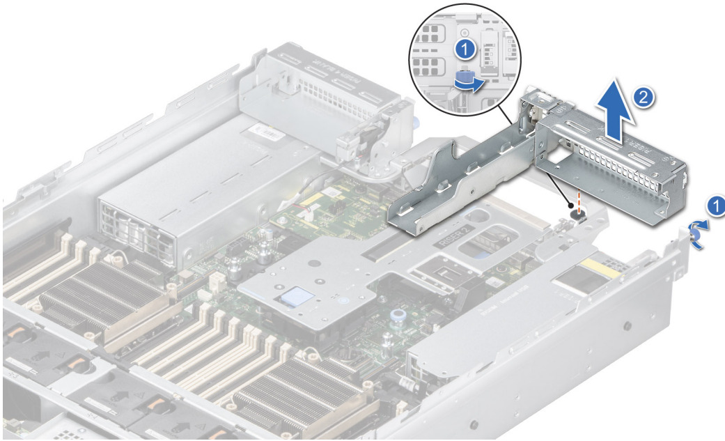
Figure 158. Removing the Riser 1 blank
