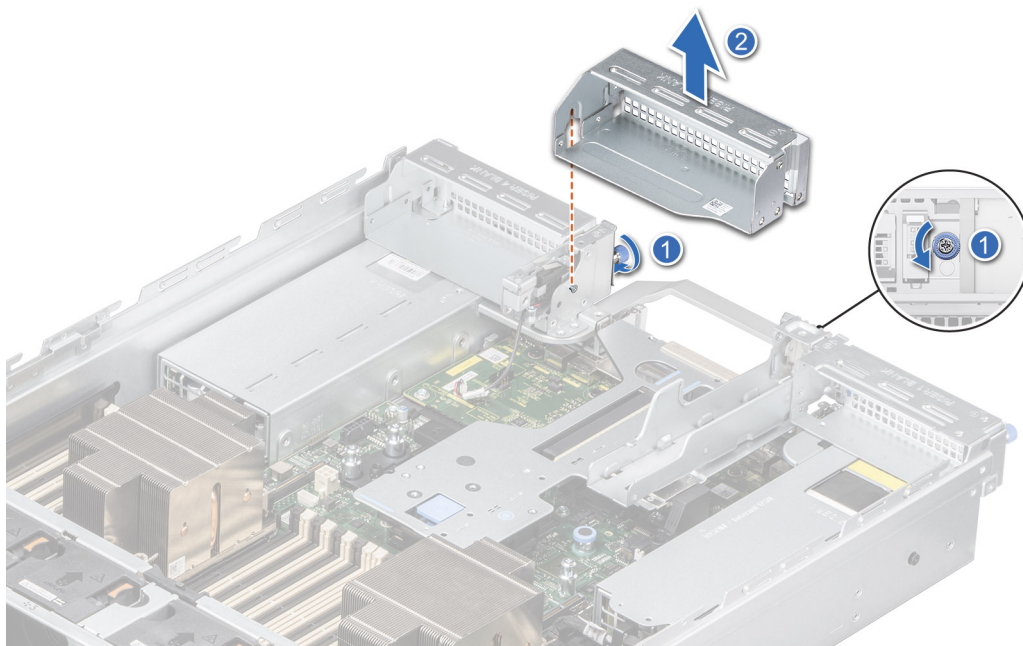
Figure 143. Removing the Riser 3 blank
