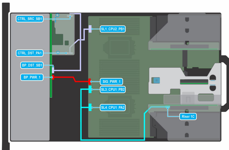
Figure 80. 16 x 2.5-inch SAS/SATA with fPERC and Riser 1C
