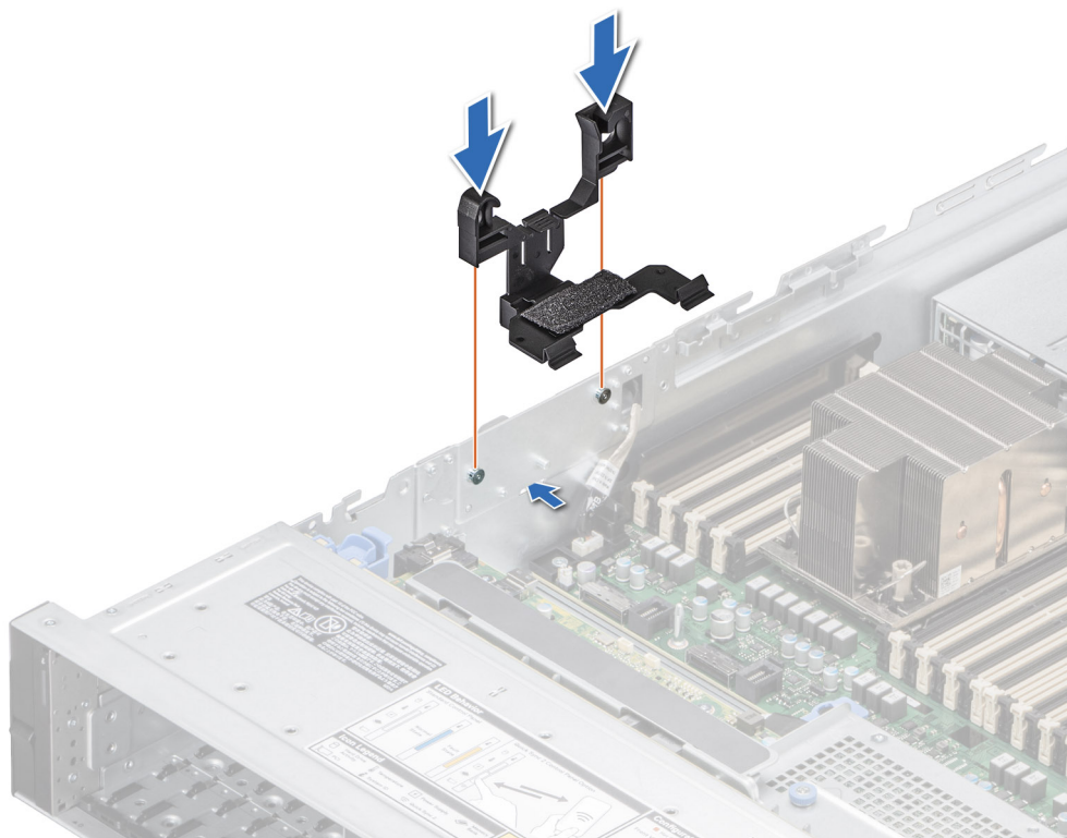
Figure 48. Installing the side wall bracket
