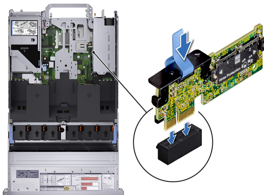
Figure 183. Installing the IDSDM module
