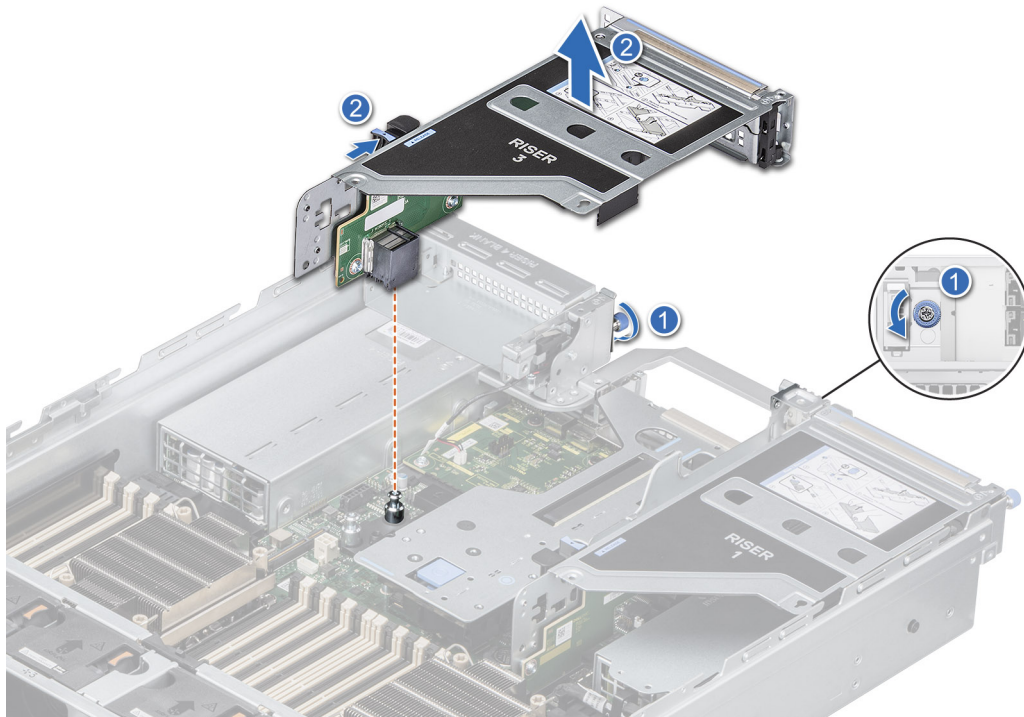
Figure 134. Removing the expansion card riser (Riser 3)
