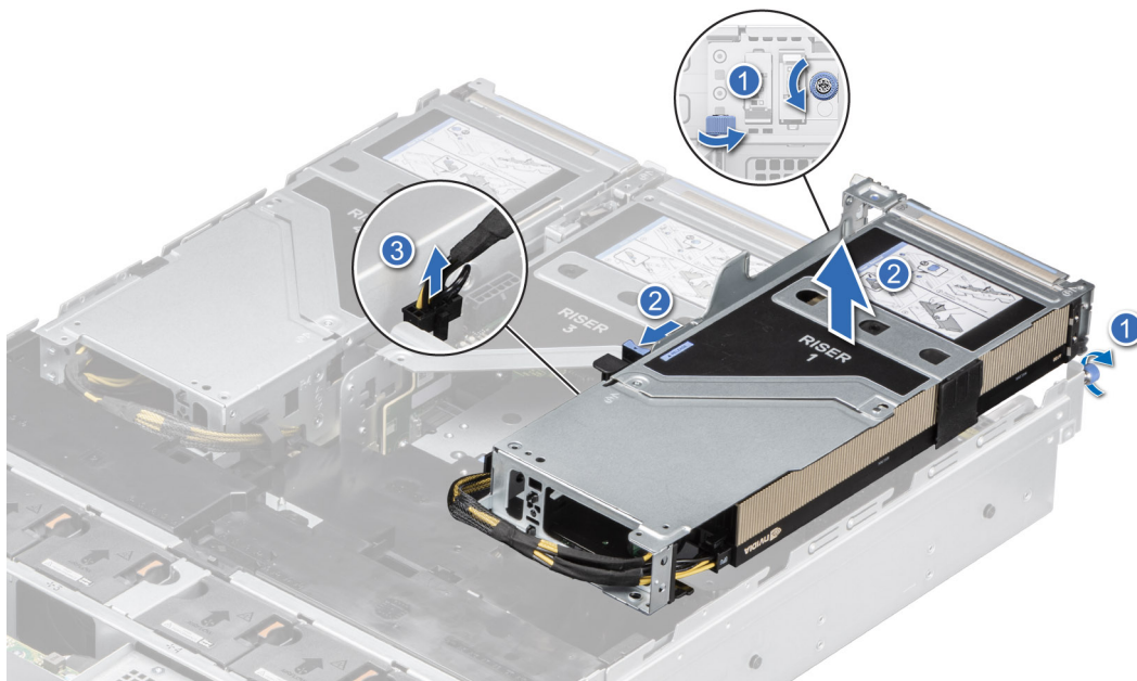
Figure 154. Removing the expansion card riser (Riser 1)
