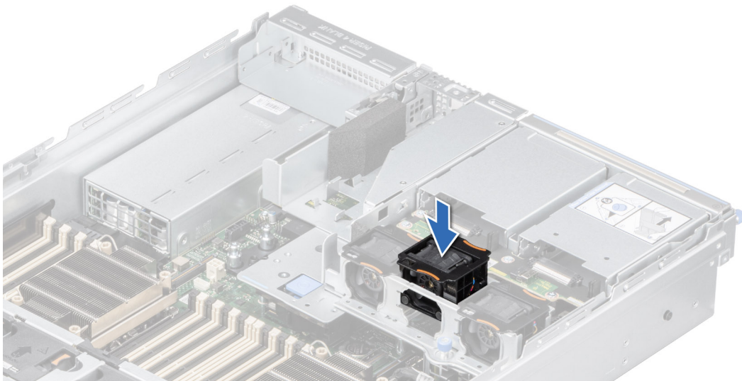
Figure 46. Installing a rear drive module cooling fan
