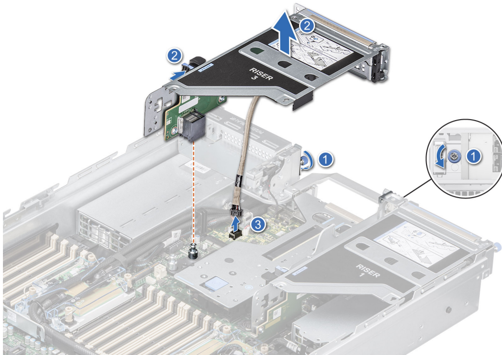
Figure 178. Disconnecting the VGA port cable
