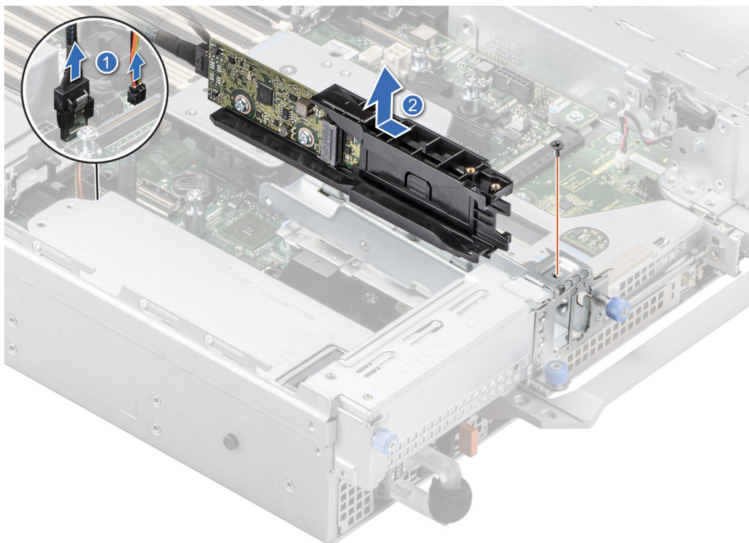
Figure 192. Removing the BOSS S2 module
