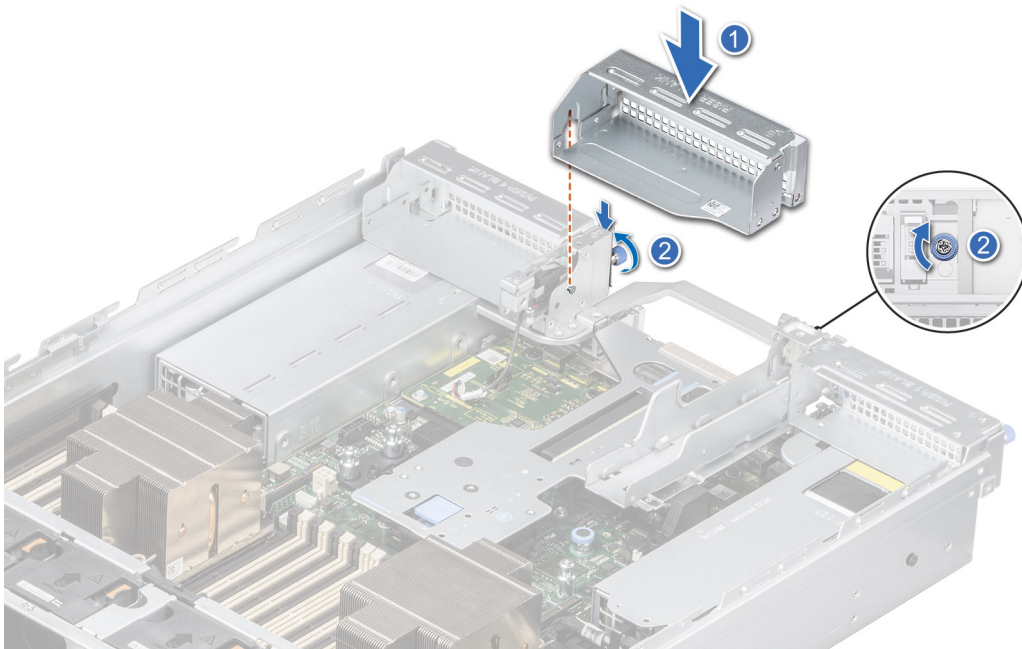
Figure 139. Installing the Riser 3 blank
