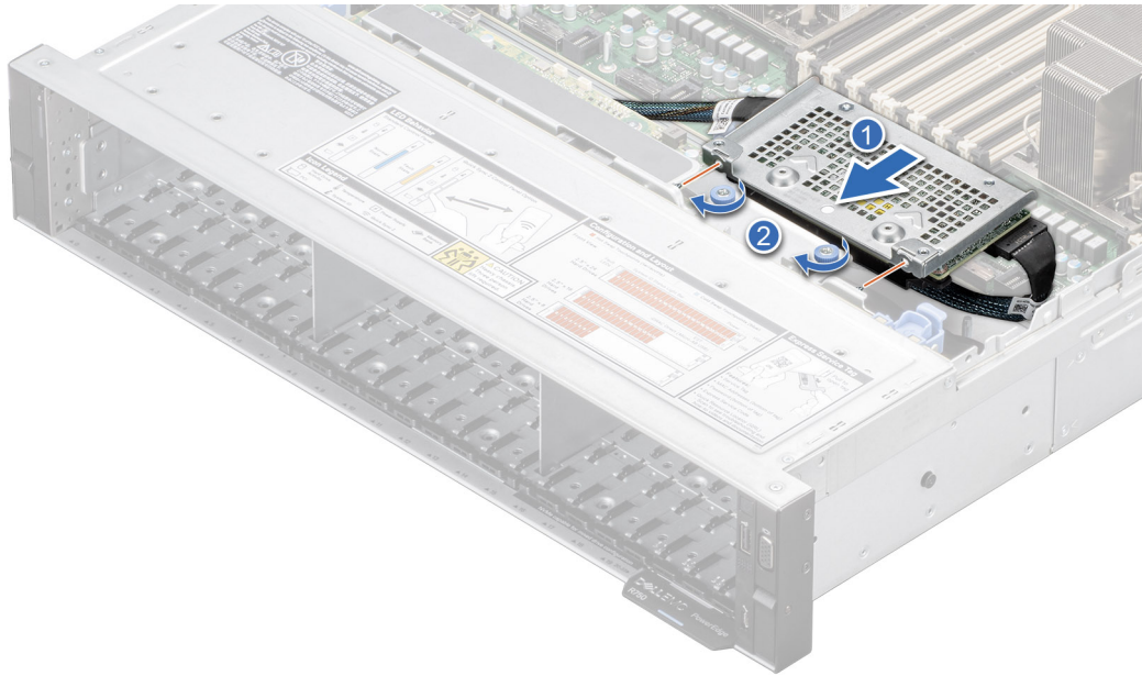
Figure 98. Installing the rear mounting front PERC module
