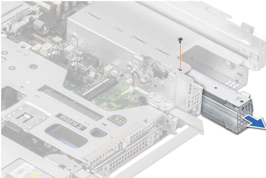
Figure 210. Removing a power supply unit adapter
