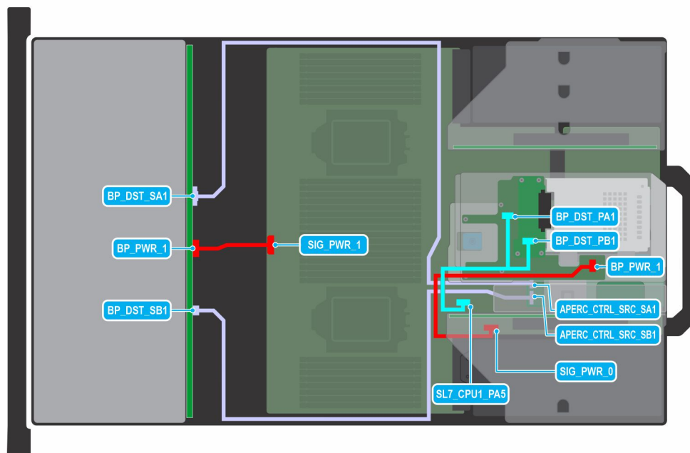
Figure 71. 12 x 3.5-inch SAS/SATA + 2 x 2.5-inch NVMe with APERC in Riser 2
