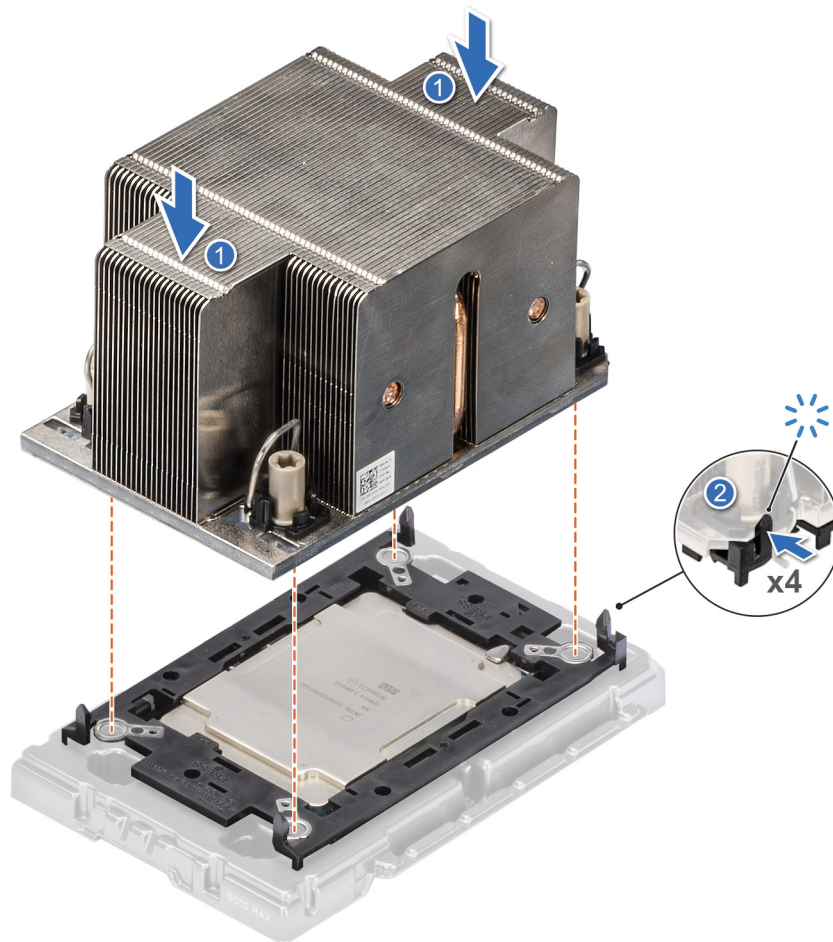
Figure 114. Installing the heat sink onto the processor
