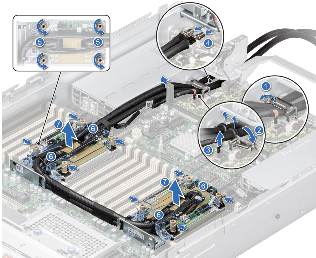
Figure 117. Removing the liquid cooling module
