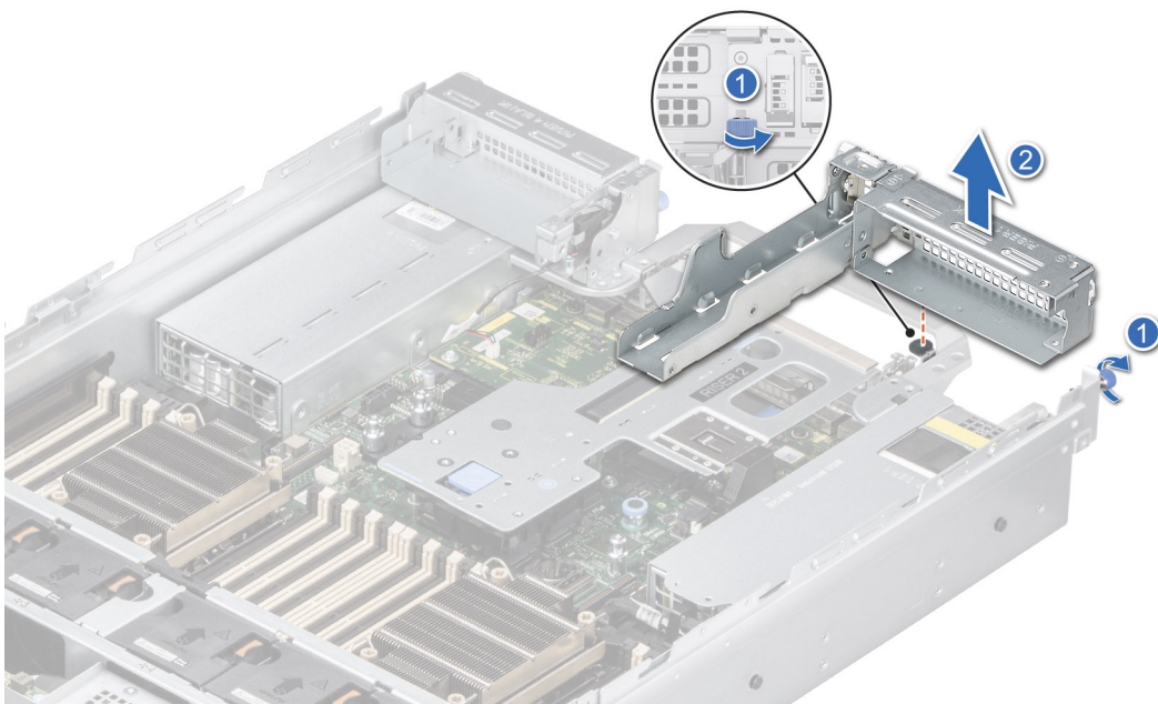
Figure 142. Removing the Riser 1 blank
