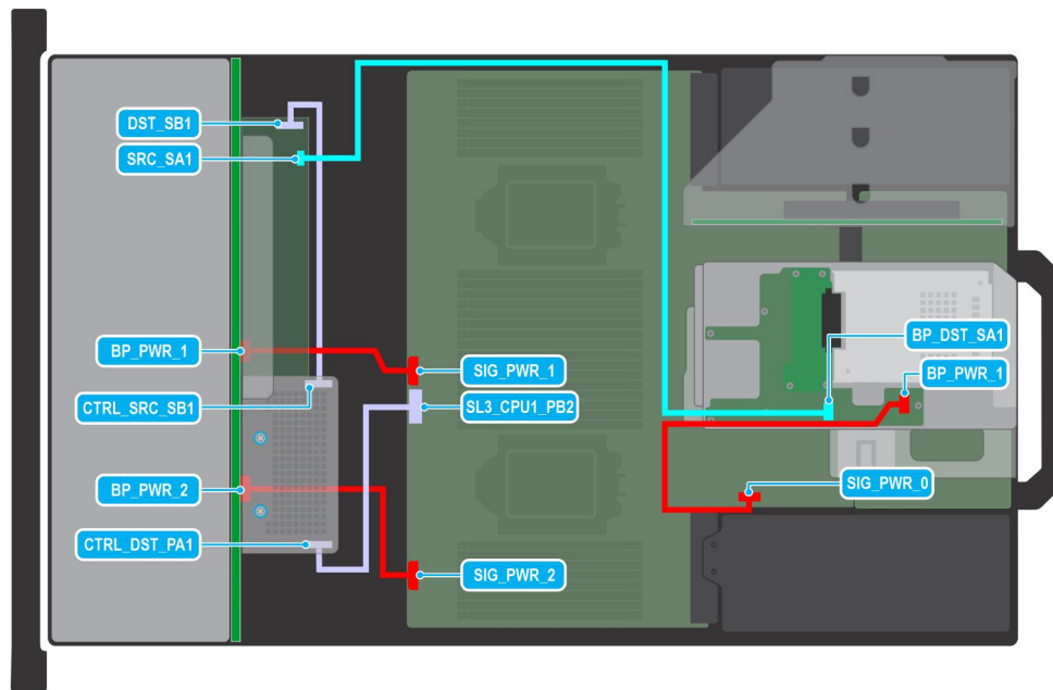
Figure 87. 24 x 2.5-inch SAS/SATA + 2 x 2.5-inch SAS with expander and fPERC
