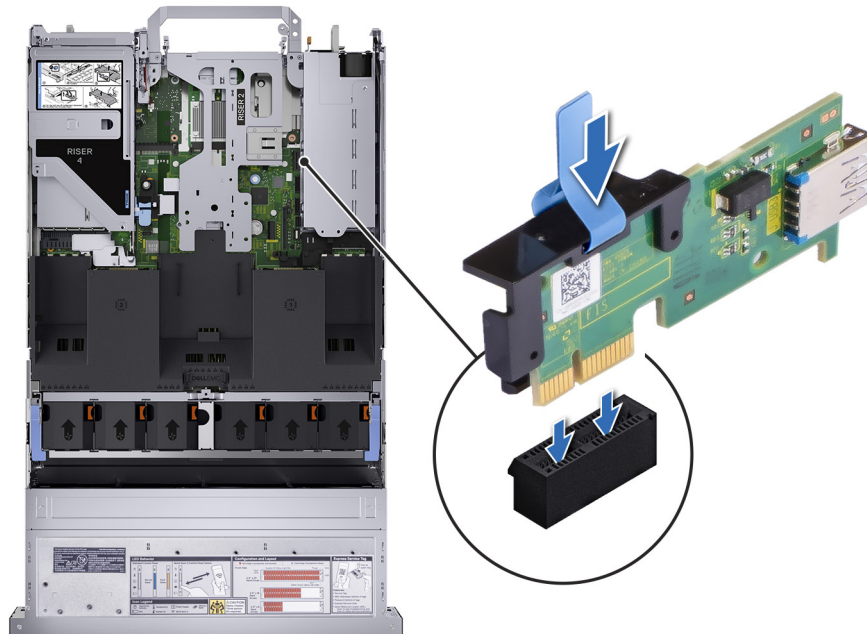
Figure 201. Installing the internal USB card
