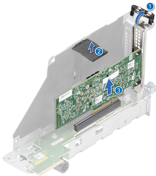
Figure 149. Removing expansion card from the expansion card riser
