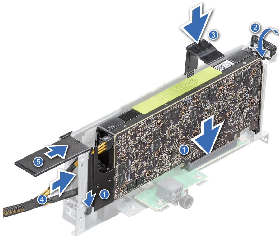
Figure 167. Installing GPU on Riser 4
