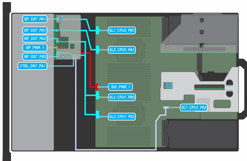
Figure 74. 8 x 2.5-inch SAS with NVMe and fPERC
