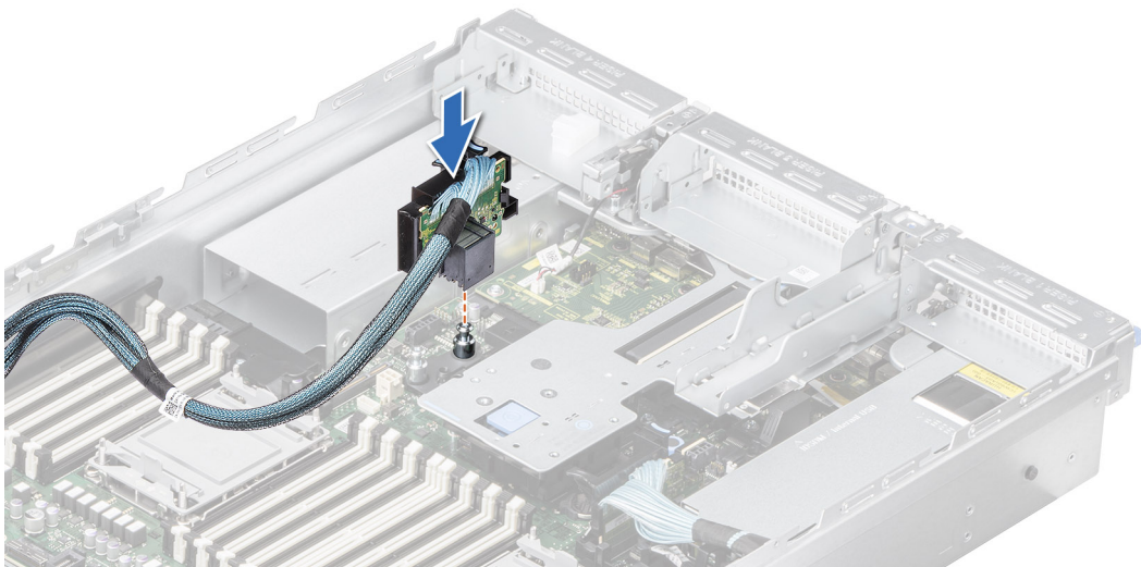
Figure 171. Installing the R3 paddle card
