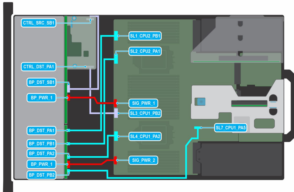
Figure 81. 16 x 2.5-inch SAS/SATA + 8 x 2.5-inch NVMe with fPERC
