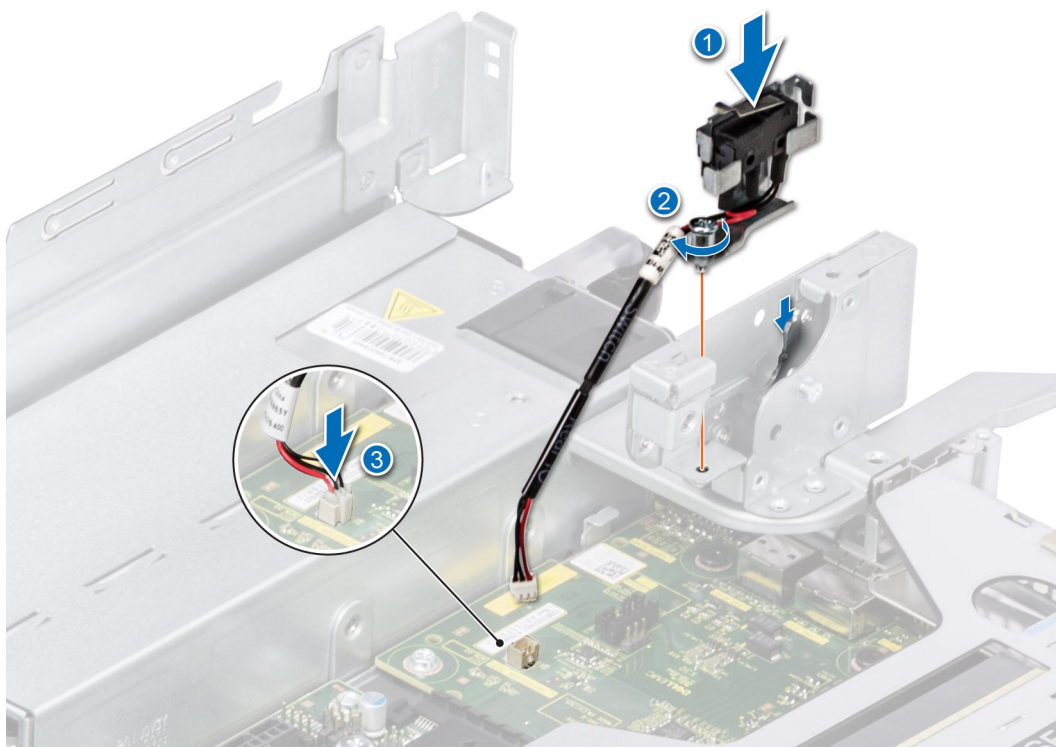
Figure 203. Installing the intrusion switch module
