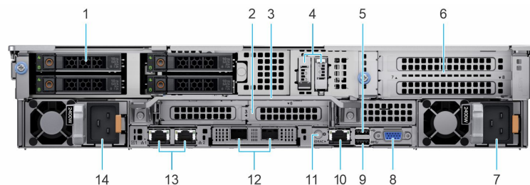
Figure 10. Rear view of the system with 4 x 2.5-inch rear drive module
