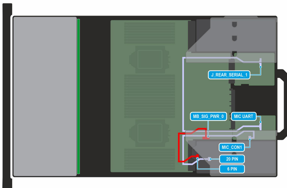
Figure 96. Management Interface Card (MIC)
