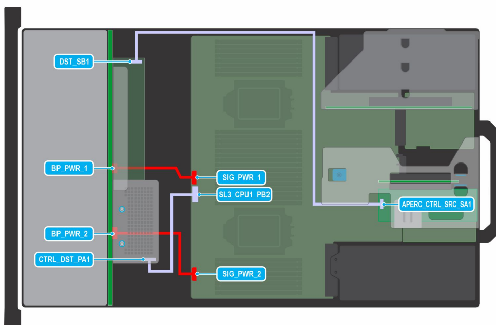
Figure 86. 24 x 2.5-inch SAS/SATA with dual controller, expander, fPERC, and APERC in Riser 2
