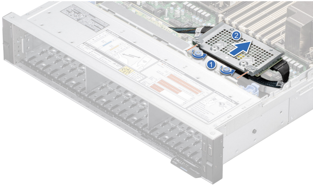
Figure 97. Removing the rear mounting front PERC module
