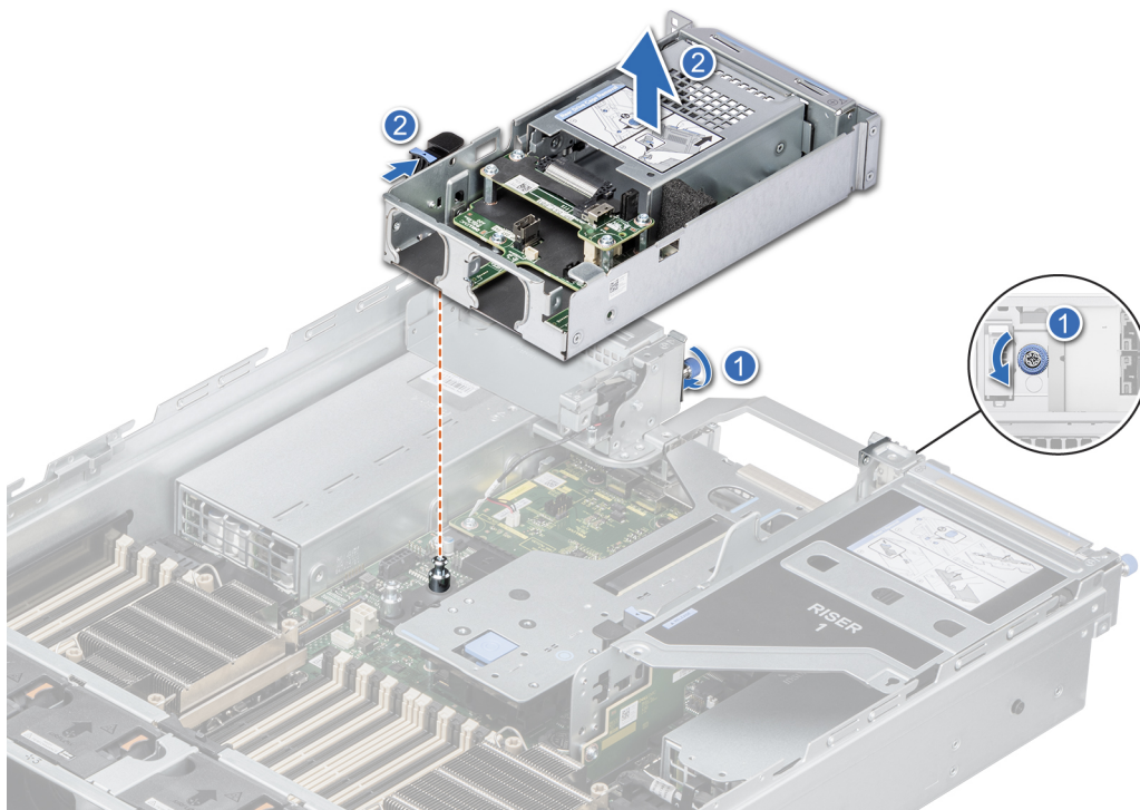
Figure 58. Removing the 2 x 2.5-inch rear drive module
