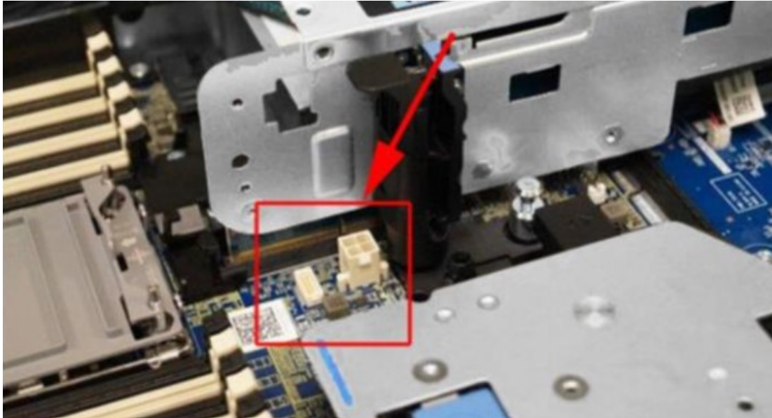
Figure 237. Connect power and signal cables to system board
