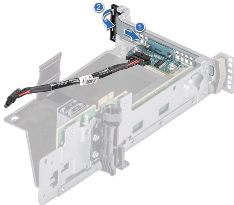
Figure 176. Installing the serial COM port
