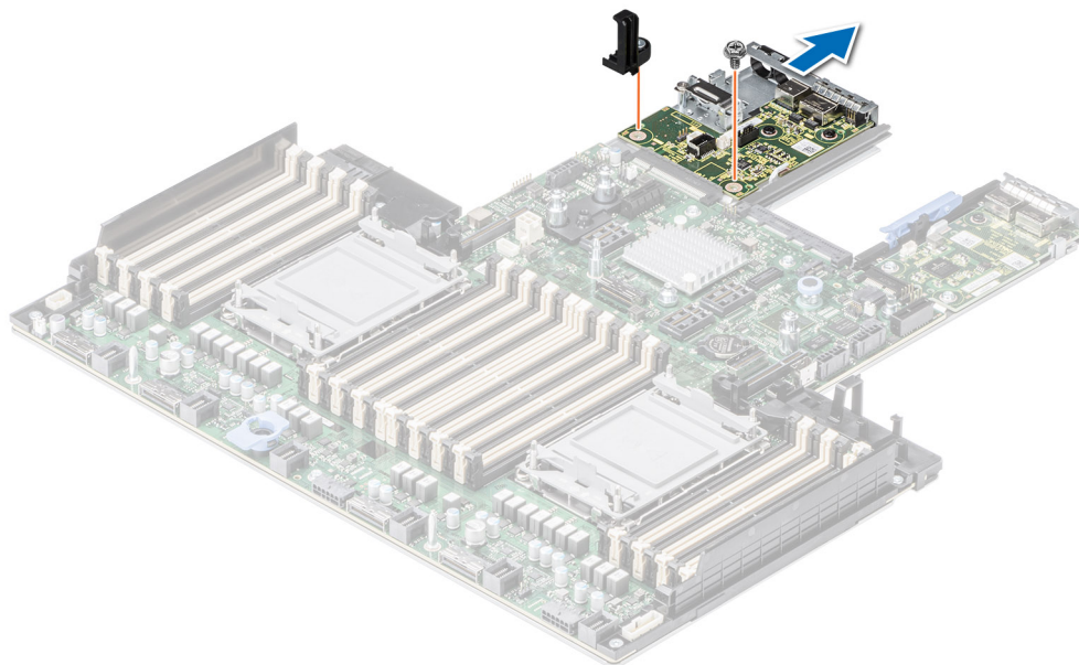
Figure 222. Removing liquid cooling rear I/O board
