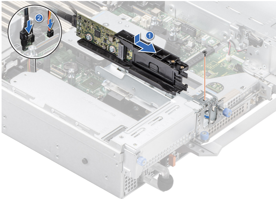
Figure 195. Installing the BOSS S2 module
