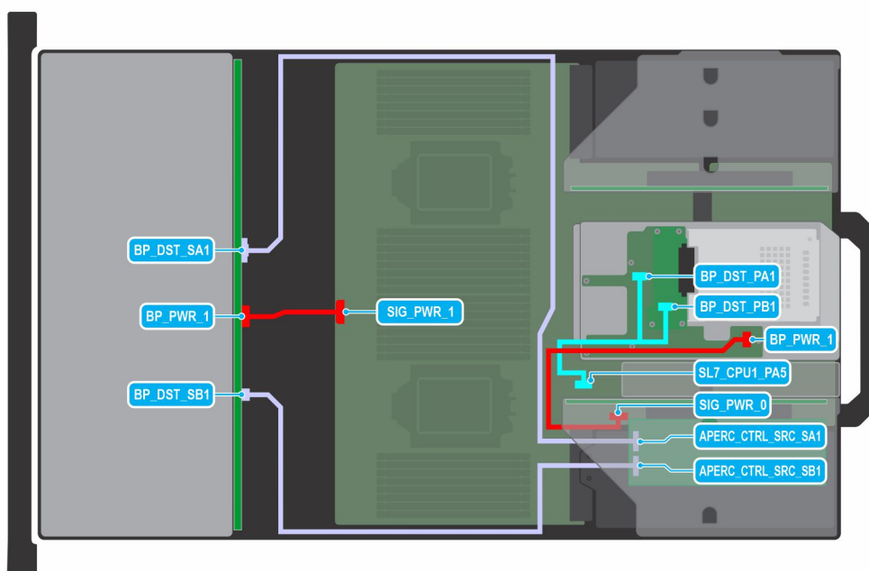
Figure 70. 12 x 3.5-inch SAS/SATA + 2 x 2.5-inch NVMe with APERC in Riser 1
