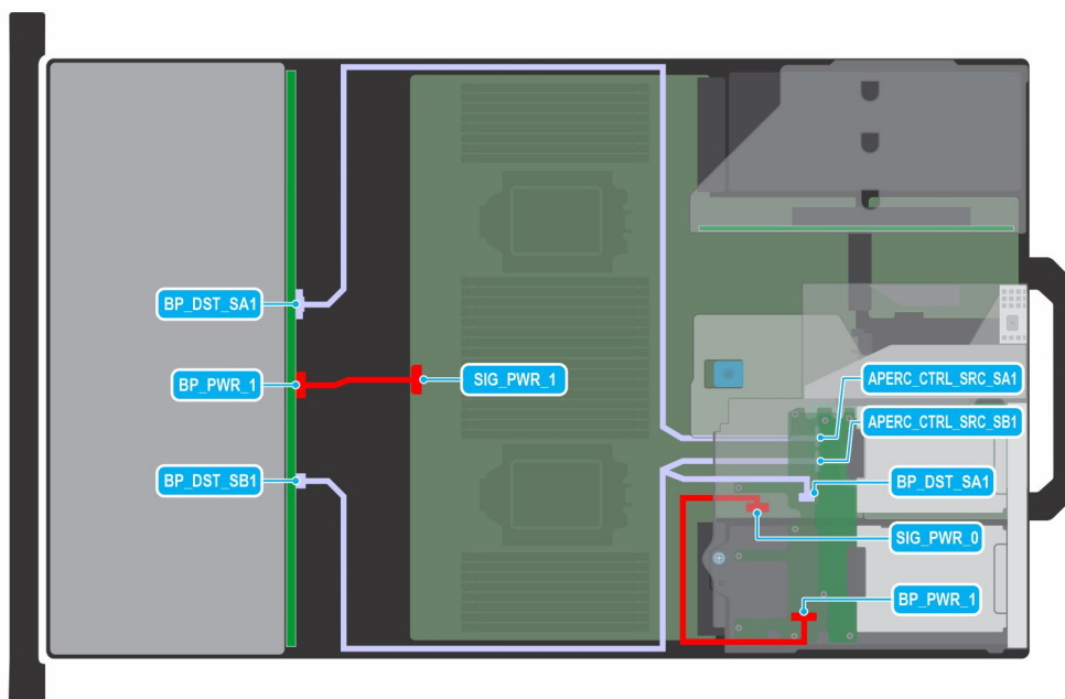
Figure 72. 12 x 3.5-inch SAS/SATA + 4 x 2.5-inch SAS/SATA with APERC in Riser 2
