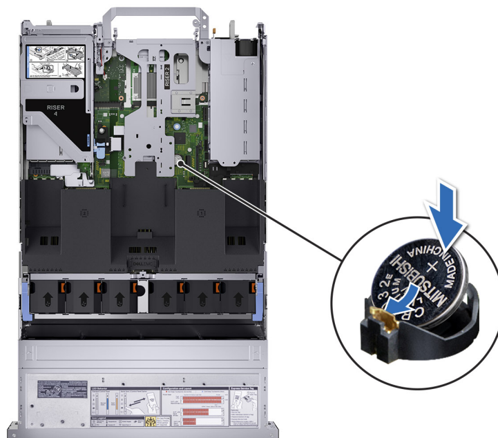
Figure 199. Installing the system battery
