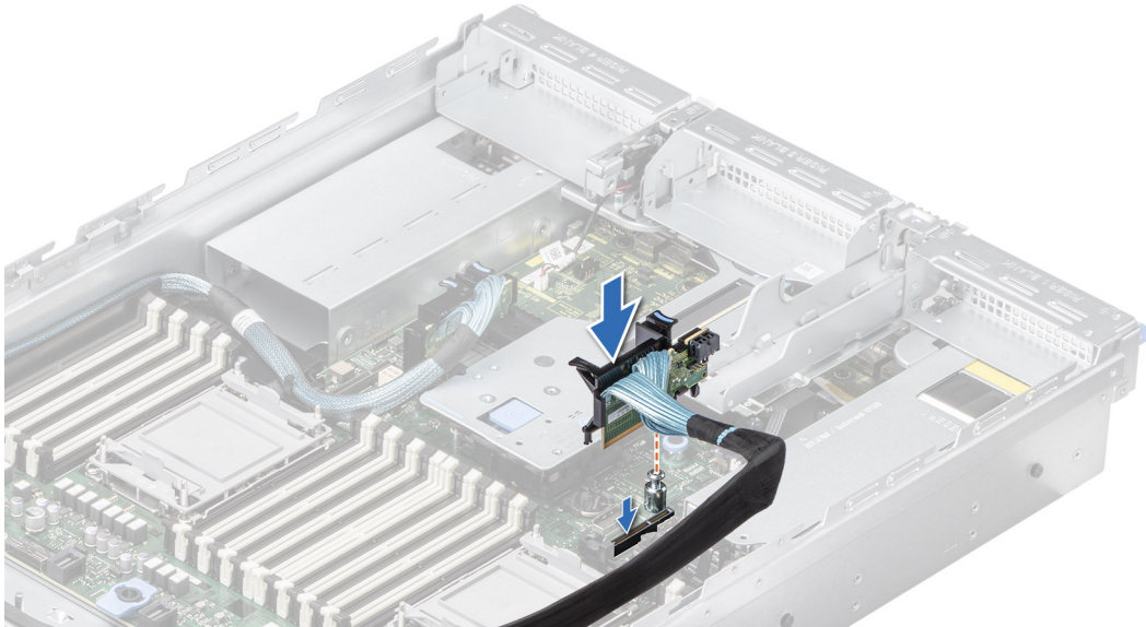
Figure 170. Installing the R1 paddle card
