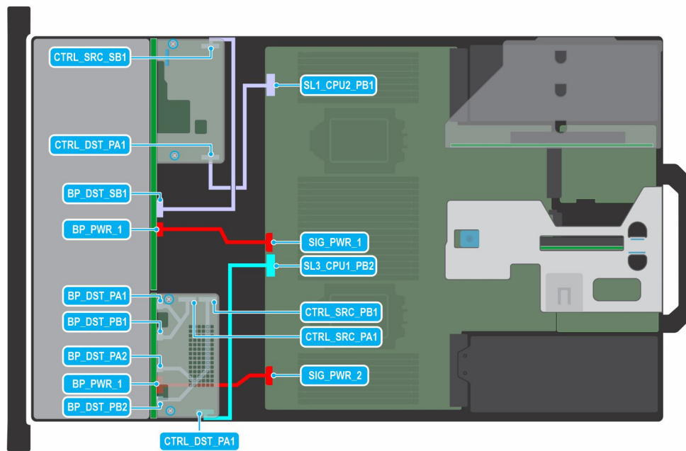
Figure 95. 16 x 2.5 SAS/SATA + 8 x 2.5 NVMe Dual PERC
