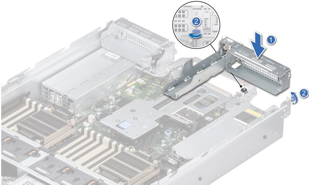
Figure 156. Installing the Riser 1 blank
