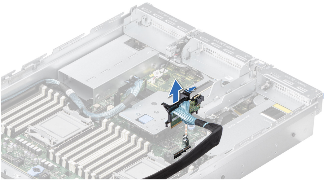
Figure 168. Removing the R1 paddle card
