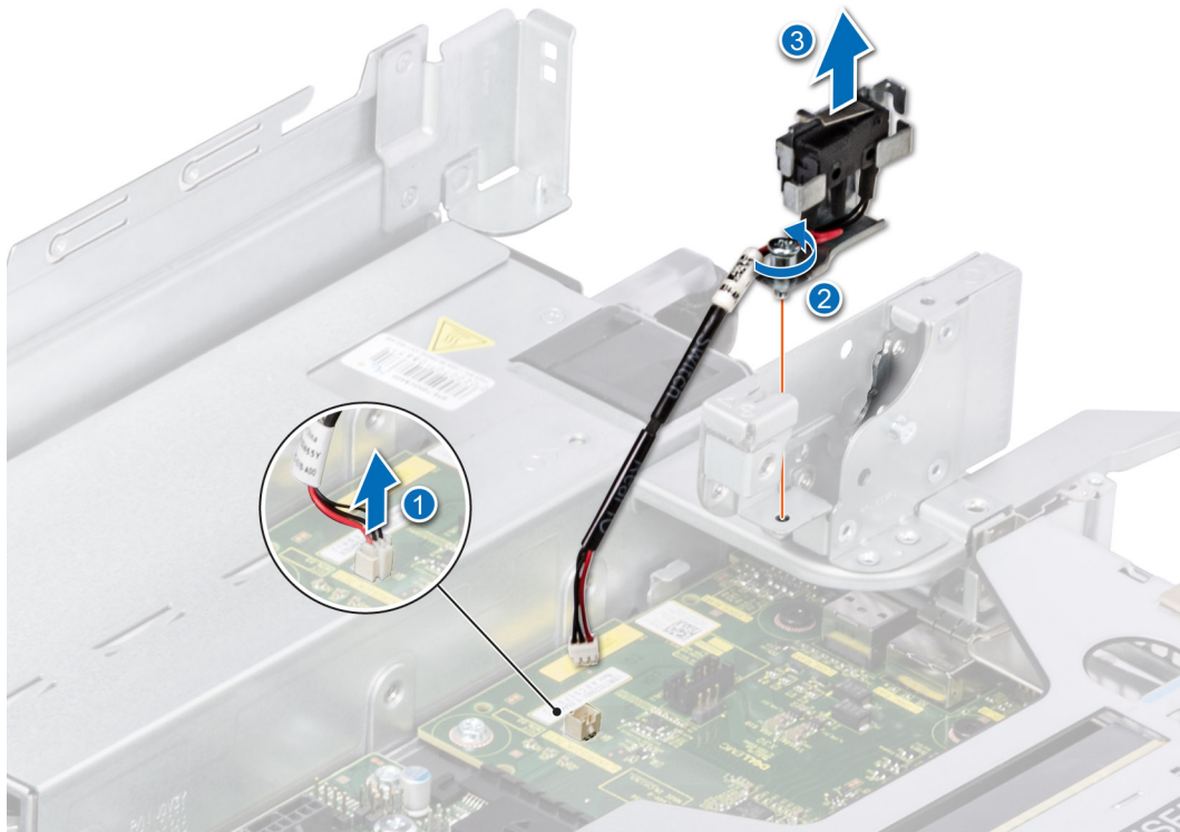
Figure 202. Removing the intrusion switch module
