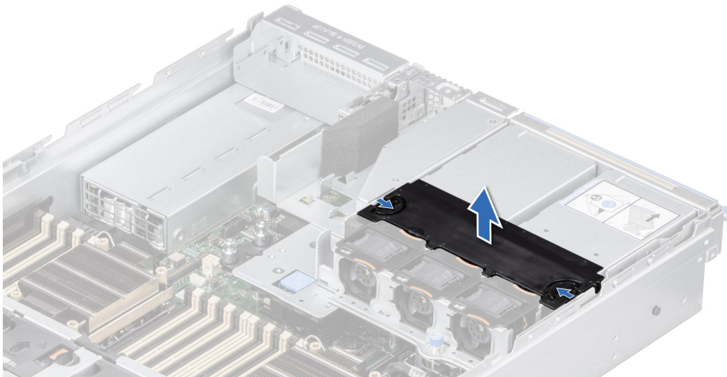
Figure 39. Removing the rear drive module air shroud
