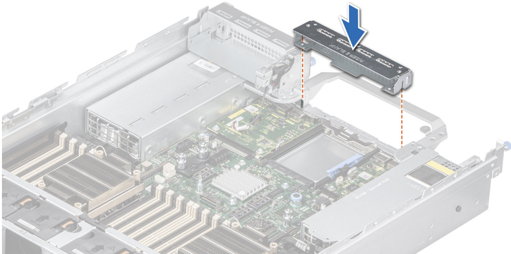
Figure 138. Installing the Riser 2 blank
