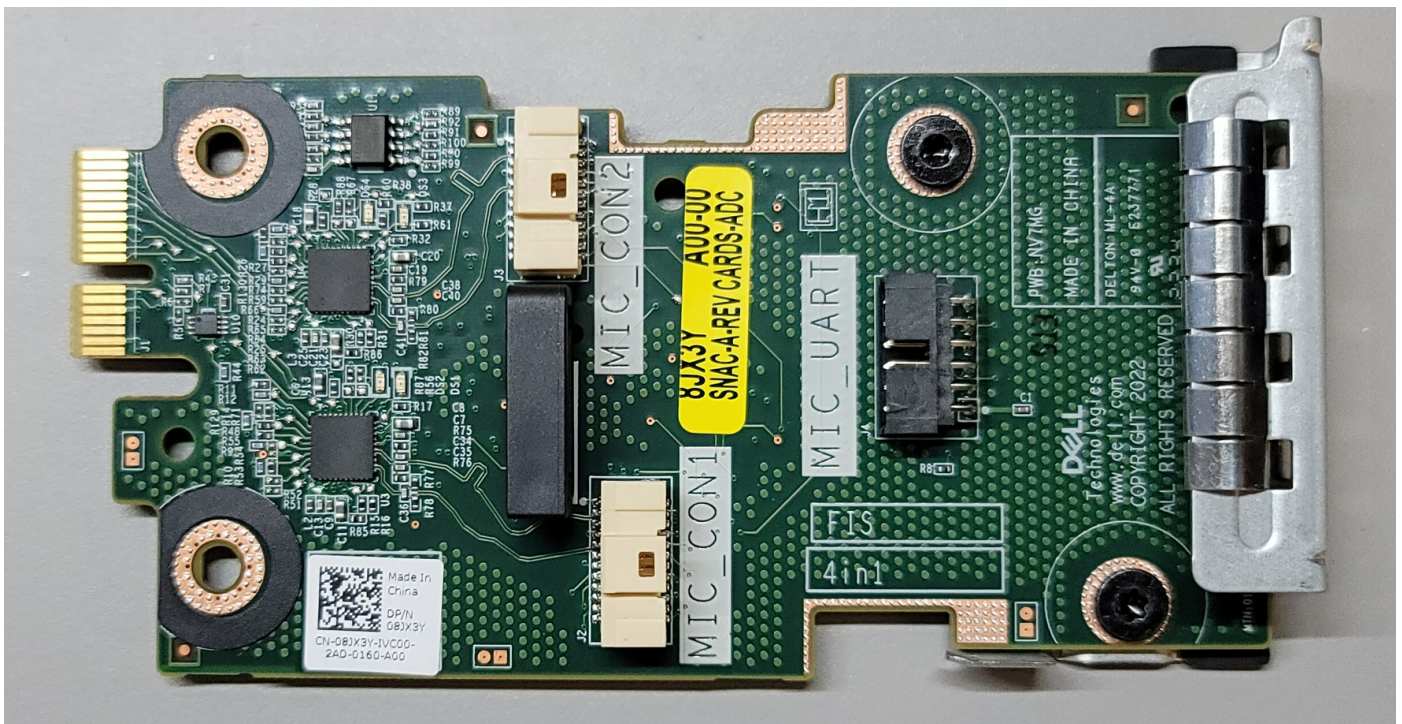
Figure 229. Management Interface Card (MIC)
