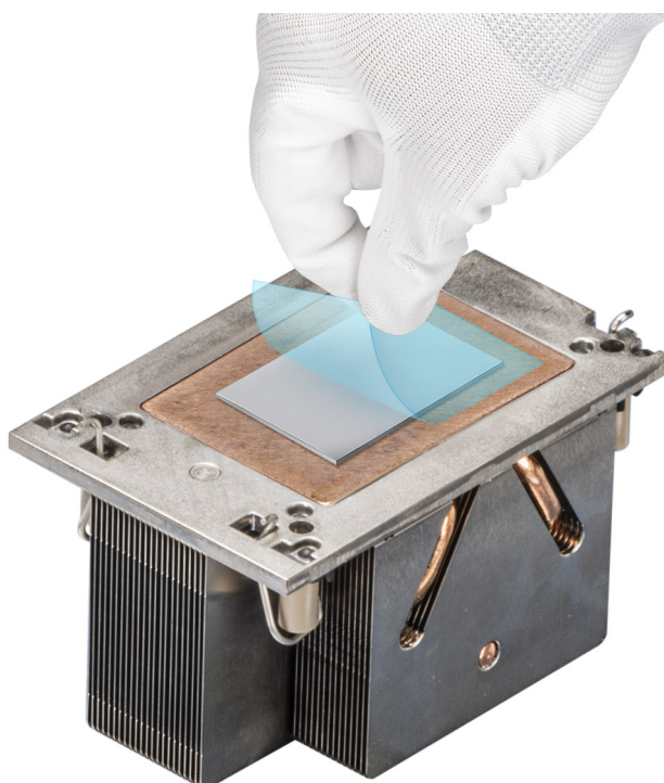
Figure 113. Removing the Thermal Interface Material (TIM) protective film
