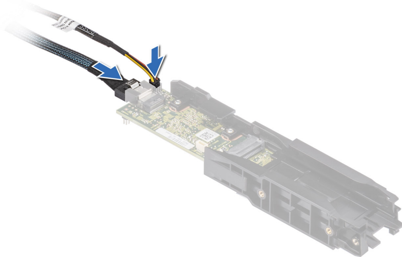
Figure 194. Connecting the BOSS S2 power and signal cables to the BOSS S2 module
