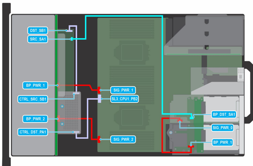
Figure 89. 24 x 2.5-inch SAS/SATA + 4 x 2.5-inch SAS with expander and fPERC
