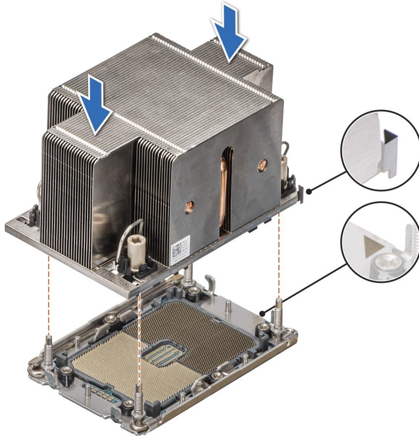
Figure 115. Installing the processor heat sink
