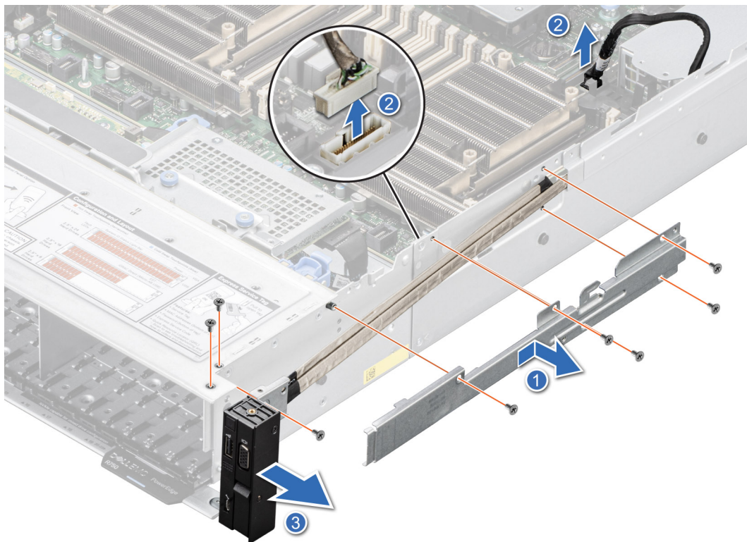
Figure 225. Removing the right control panel
