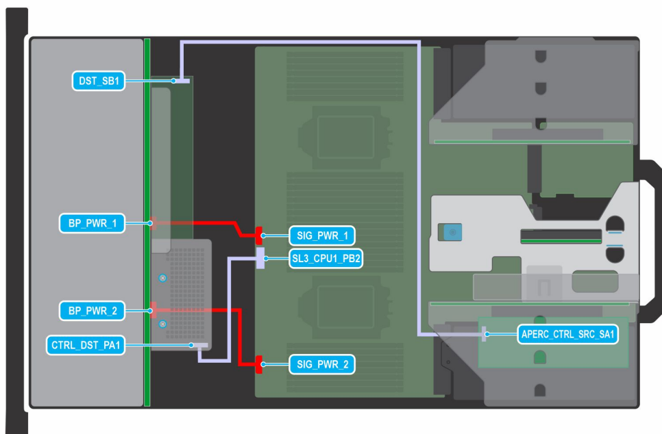
Figure 85. 24 x 2.5-inch SAS/SATA with dual controller, expander, fPERC, and APERC in Riser 1
