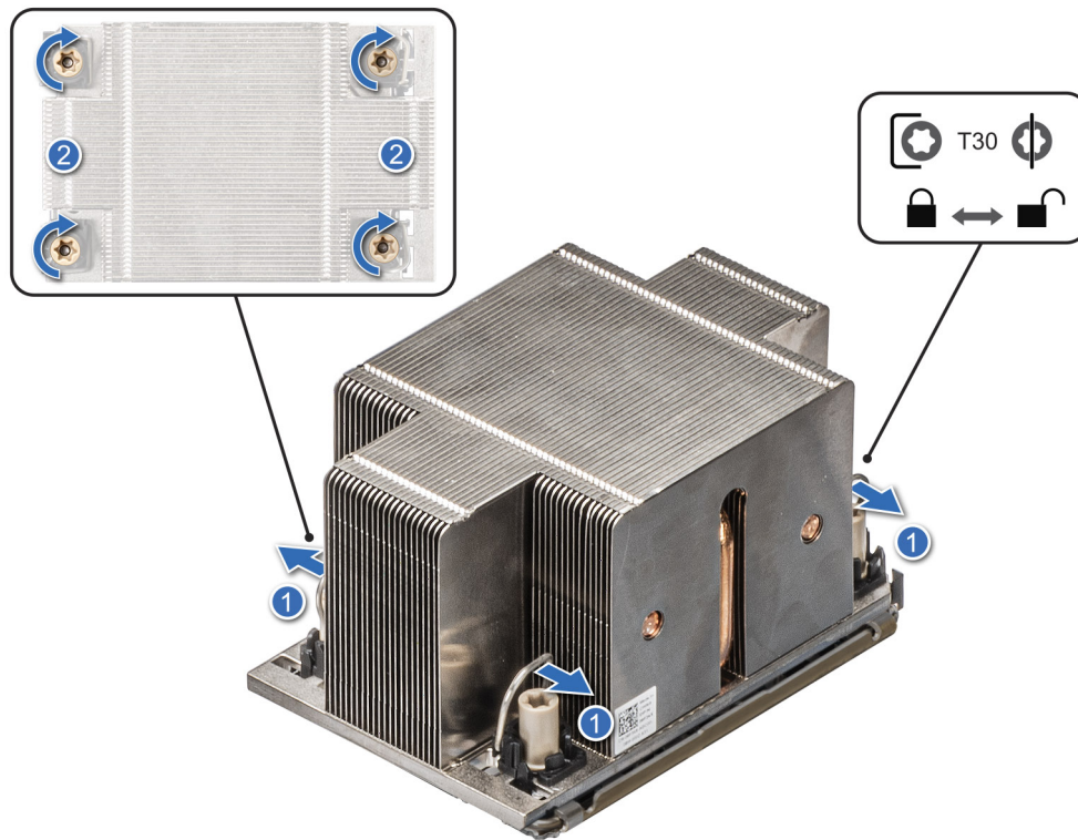
Figure 116. Set the anti-tilt wires to the locked position and tightening the nuts
