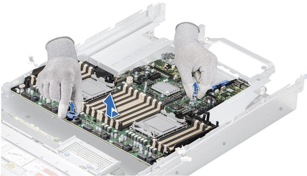
Figure 219. Removing the system board
