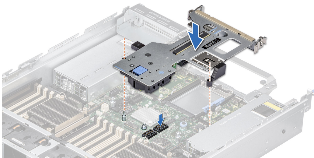
Figure 145. Installing the expansion card riser (Riser 2)
