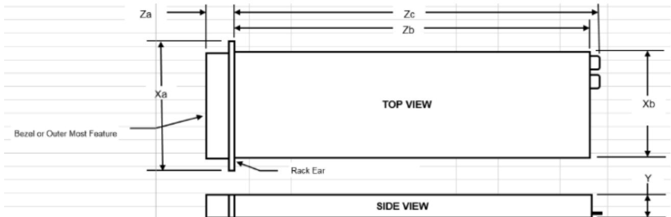
Figure 36. Chassis dimensions
