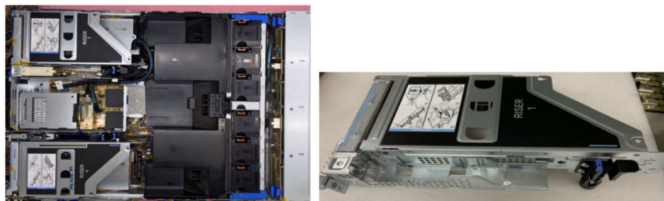
Figure 30. Shroud/HSK/Riser Cage
