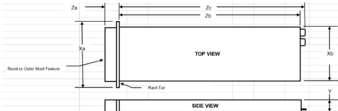
Figure 27. Chassis dimensions
