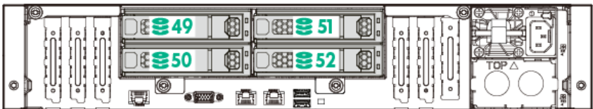
Drive numbering – Four-bay LFF hot-plug rear drive numbering
