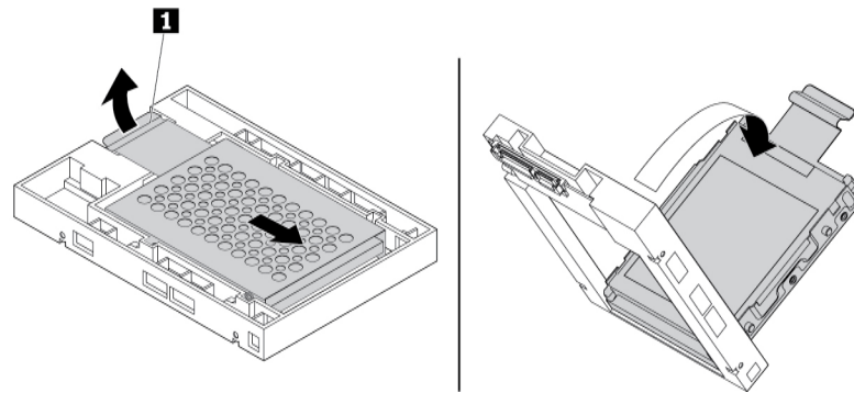
Figure 65. Removing the metal bracket from the plastic frame of the converter
