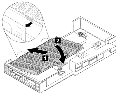
Figure 93. Installing the heat sink onto the M.2 solid-state drive holder
