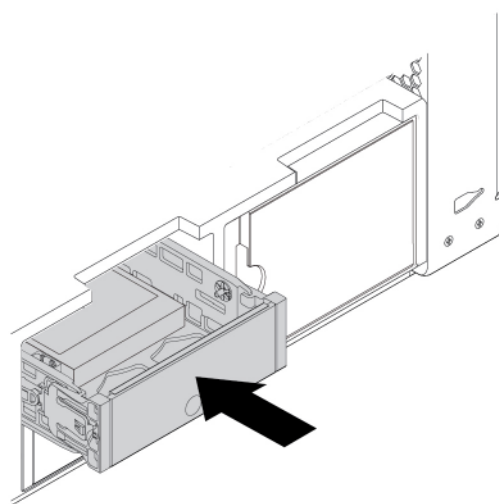
Figure 61. Installing the type 2 storage drive bracket
