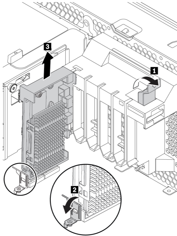
Figure 87. Removing the M.2 solid-state drive holder
