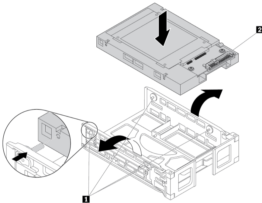
Figure 70. Installing the converter into the type 1 bracket
