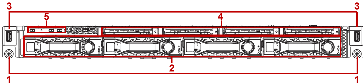
Figure 1-4. Hybrid 3.5" + 2.5" Storage Drive System Front View
