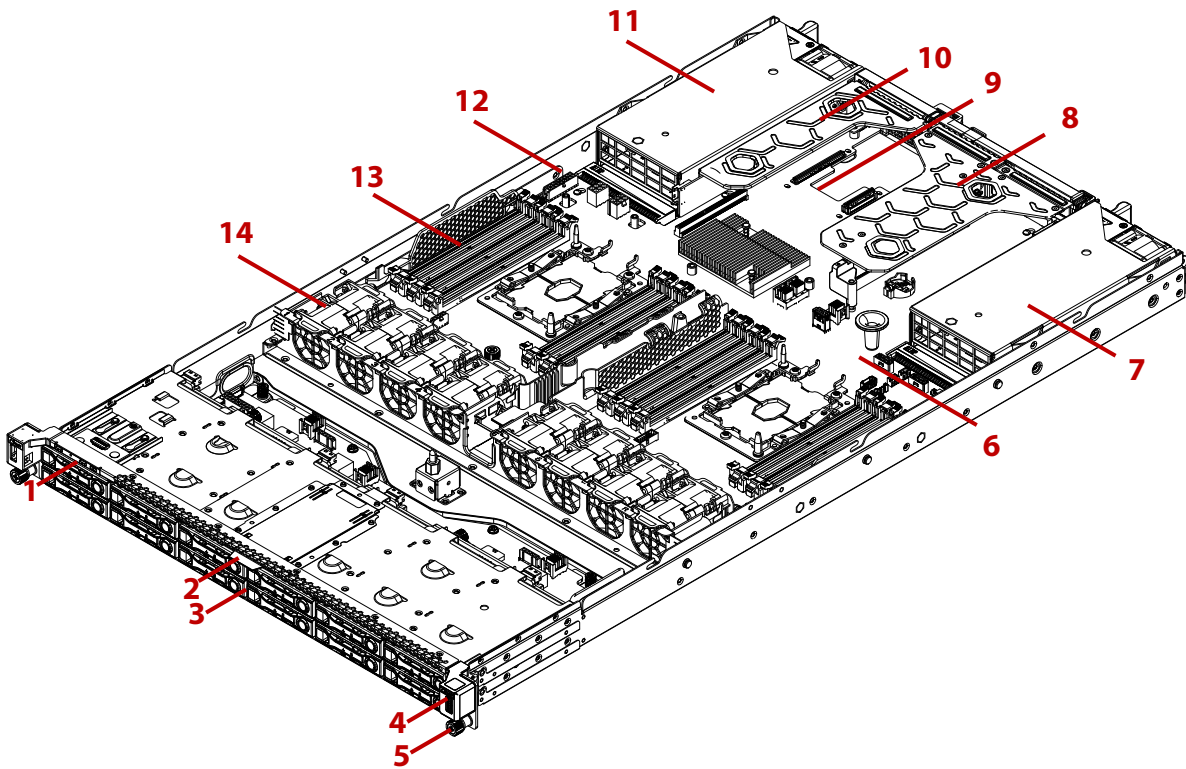
Figure 1-1. 2.5" Storage Drive System Component Overview
