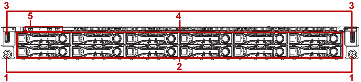
Figure 1-3. 2.5" Storage Drive System Front View
