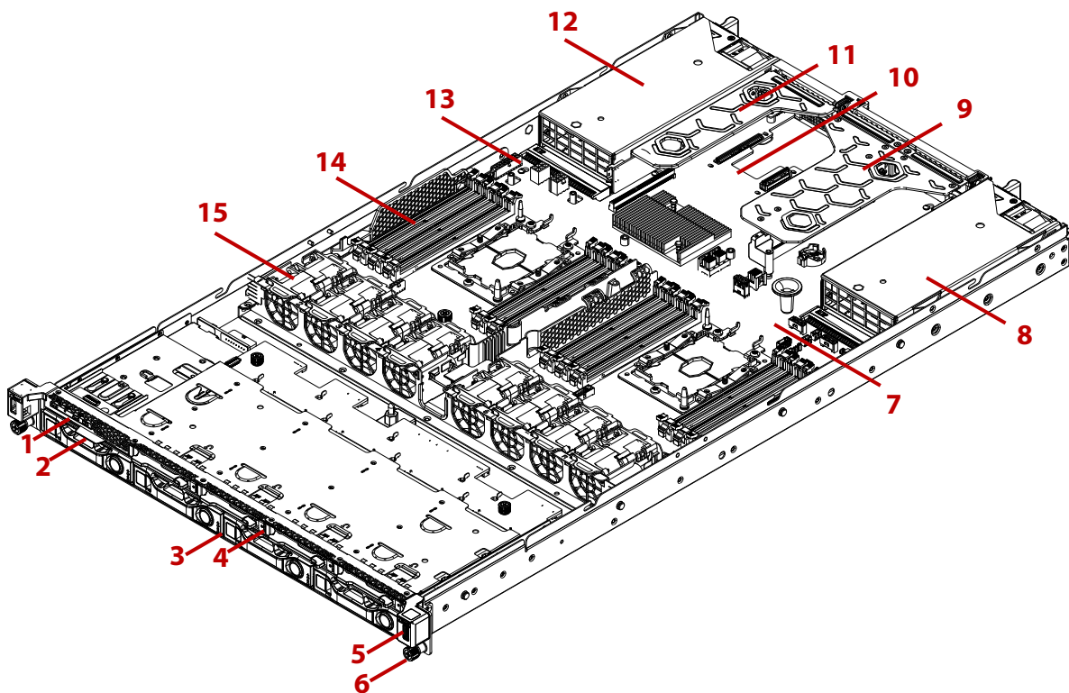
Figure 1-2. Hybrid 3.5" + 2.5" Storage Drive System Component Overview
