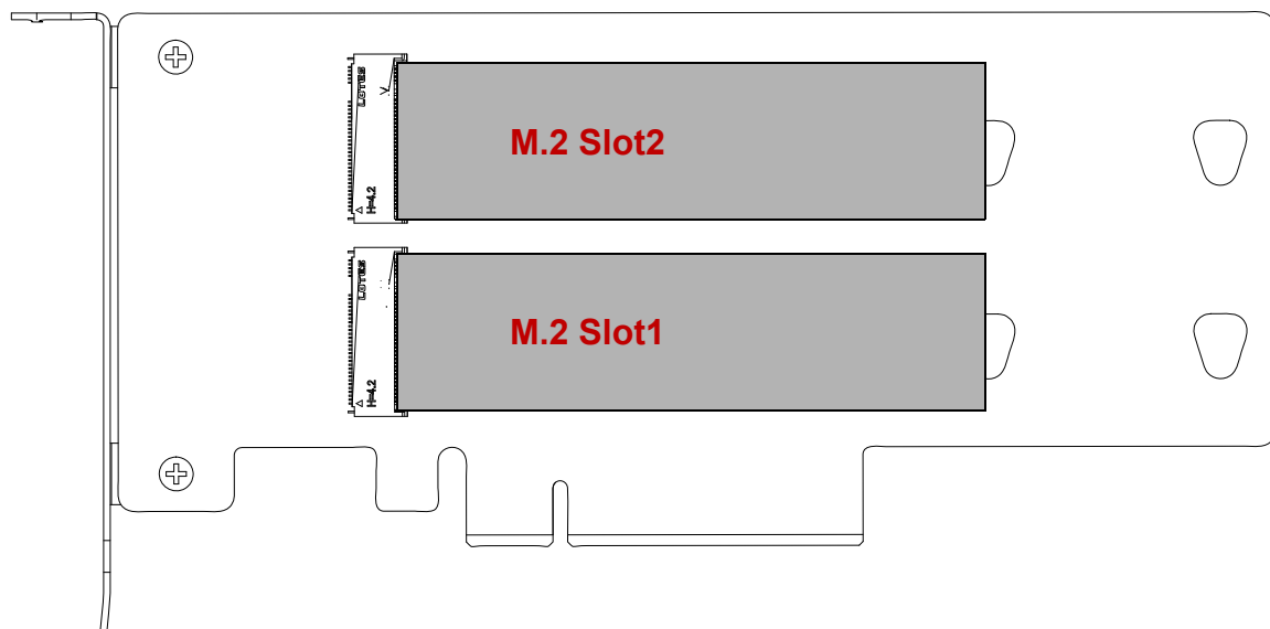
Figure 1-11. M.2 Slot Number
