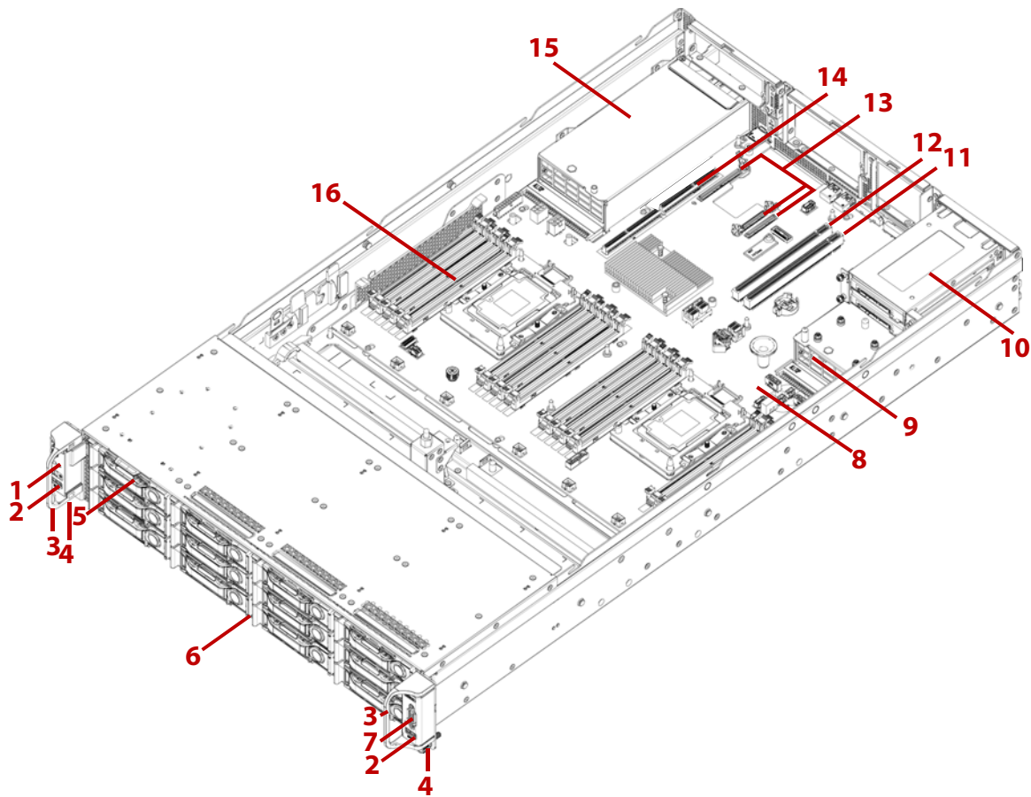
Figure 1-2. 3.5" Storage Drive System Component Overview
