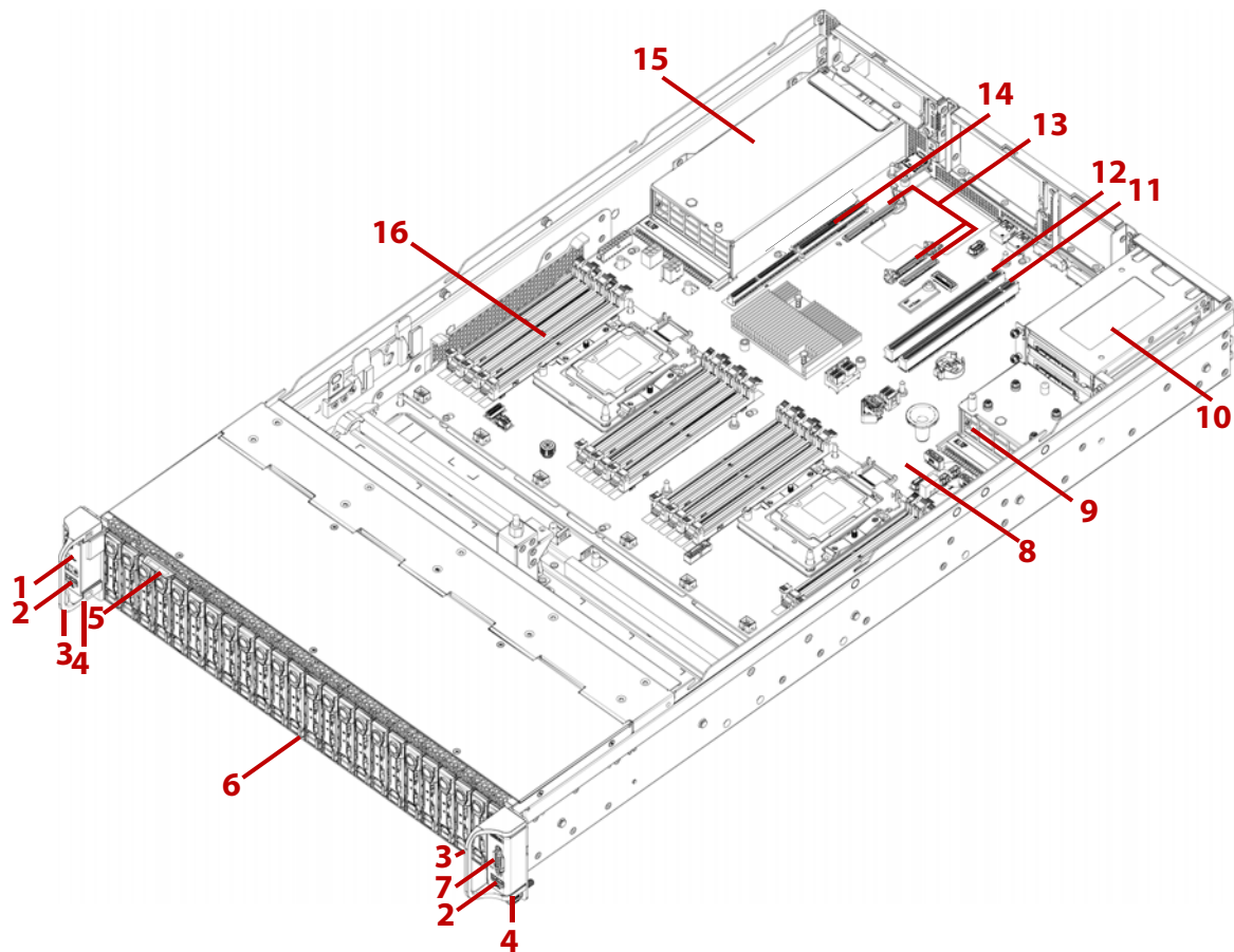
Figure 1-1. 2.5" Storage Drive System Component Overview
