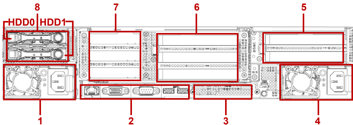
Figure 1-7. System Rear View
