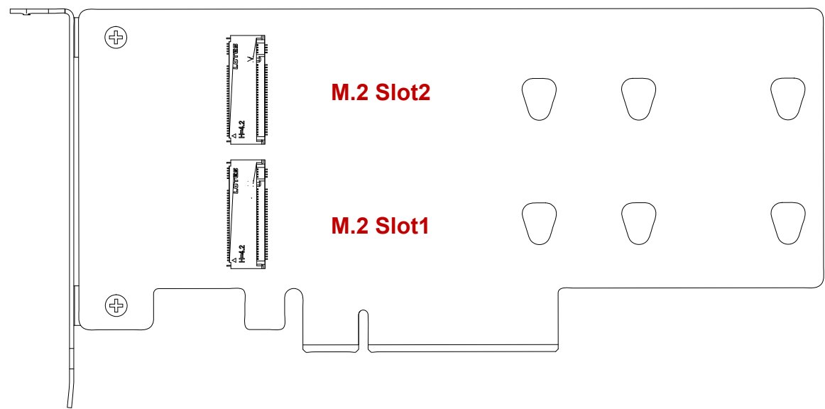
Figure 1-5. M.2 Slot Number
